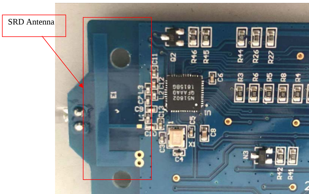
EUT –PCB-1 Top Chip View
