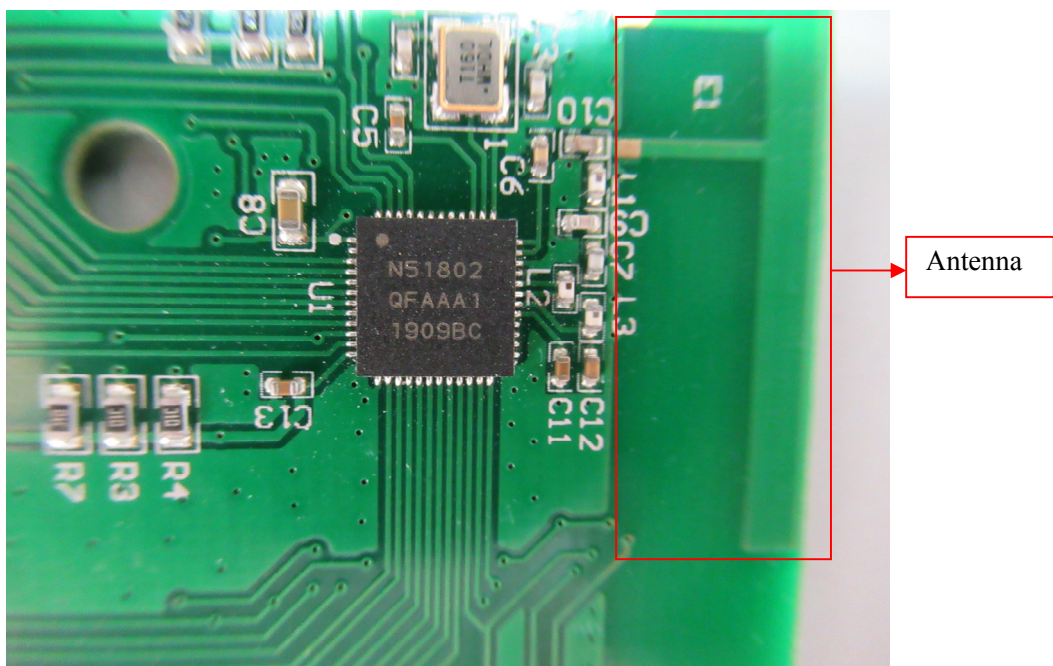
EUT – PCB Top Chip View
