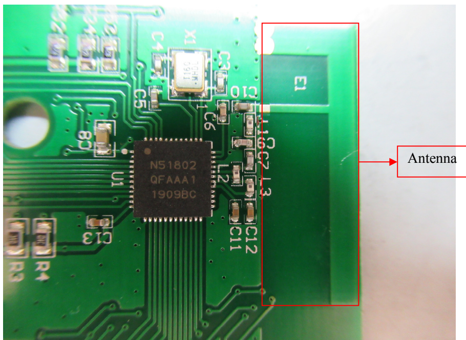
EUT – PCB Bottom Chip View
