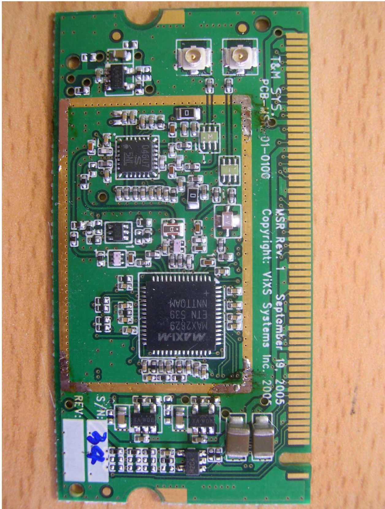
<Photograph 4: Rear View - RF module>
