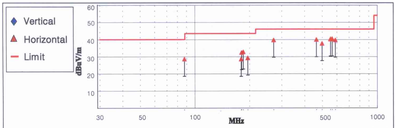
< Fig 6-2. Radiated emission result >
