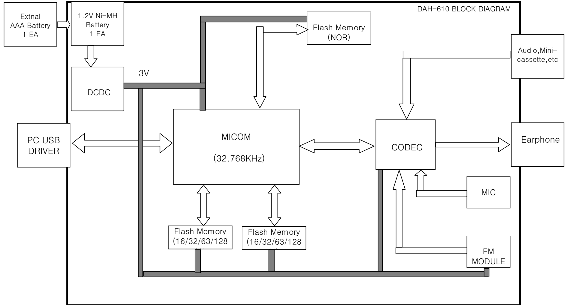
DAH-610 BLOCK DIAGRAM
