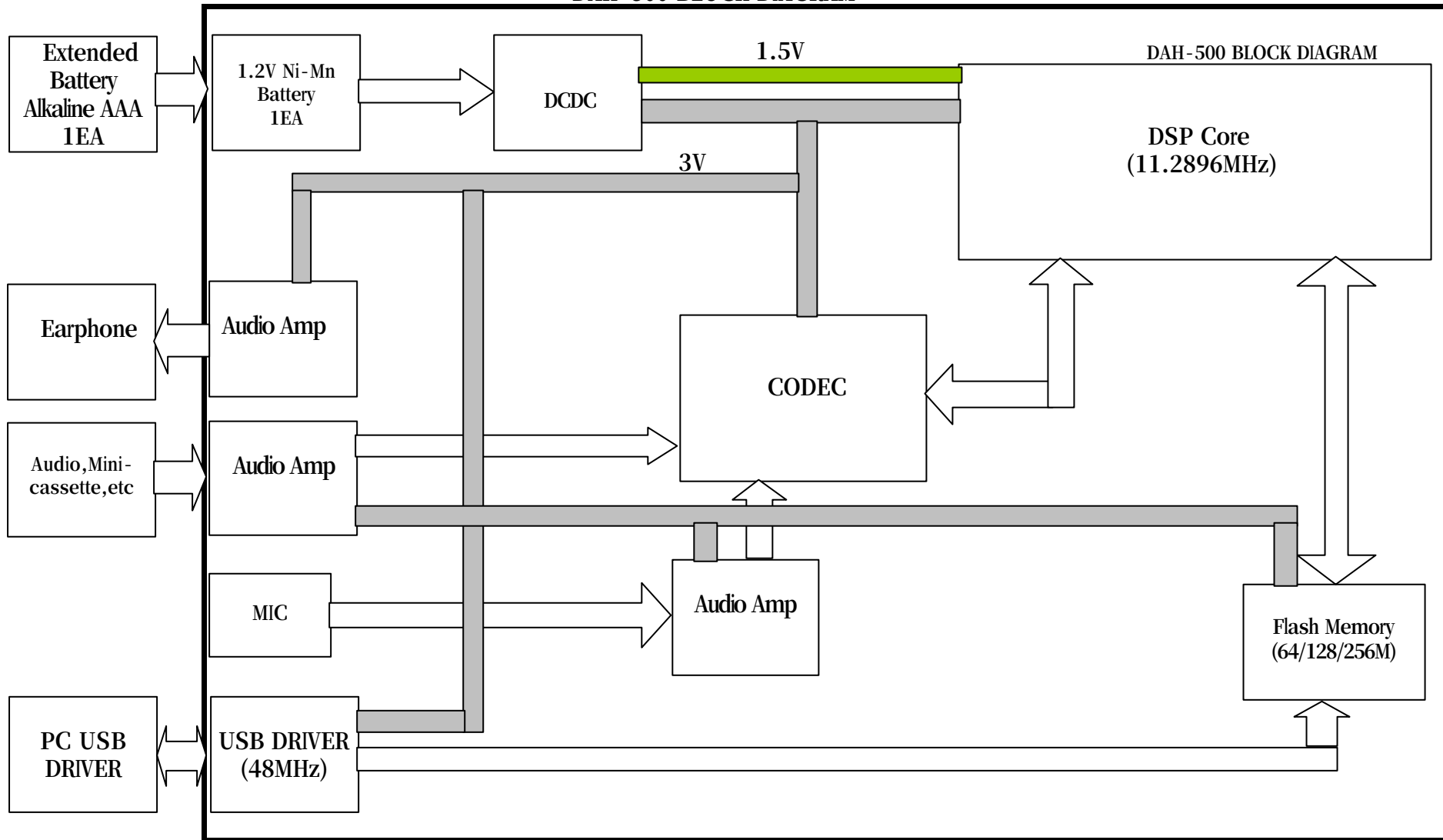
DAH-500 BLOCK DIAGRAM
