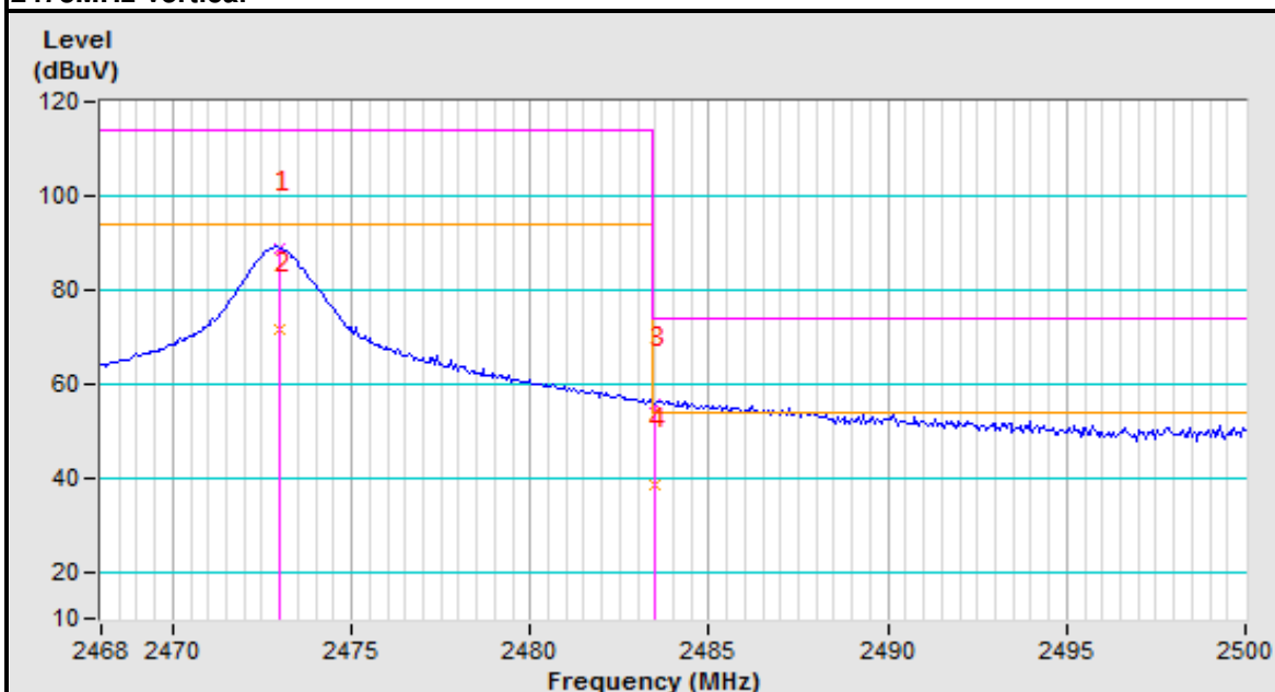
2473MHz Vertical
