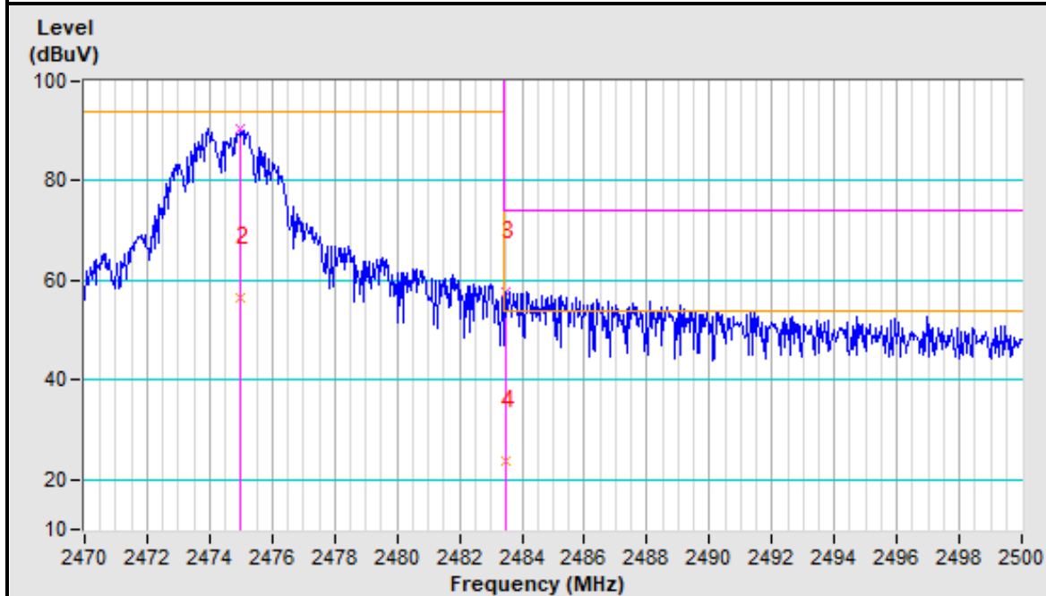
2475MHz Vertical
