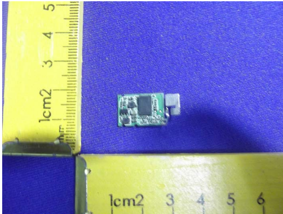
Figure 2 The EUT-Inside View
