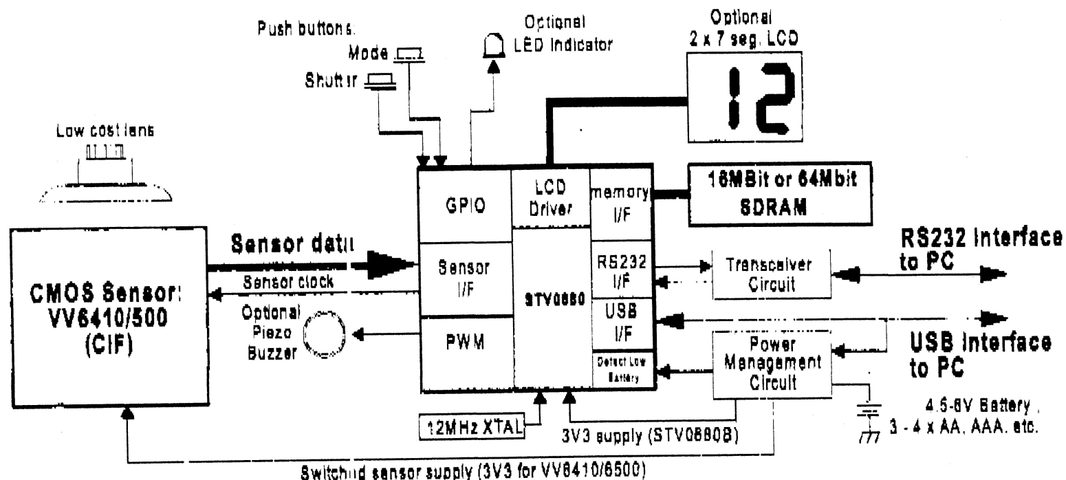
Figure 1 : Typical camera system block diagram
