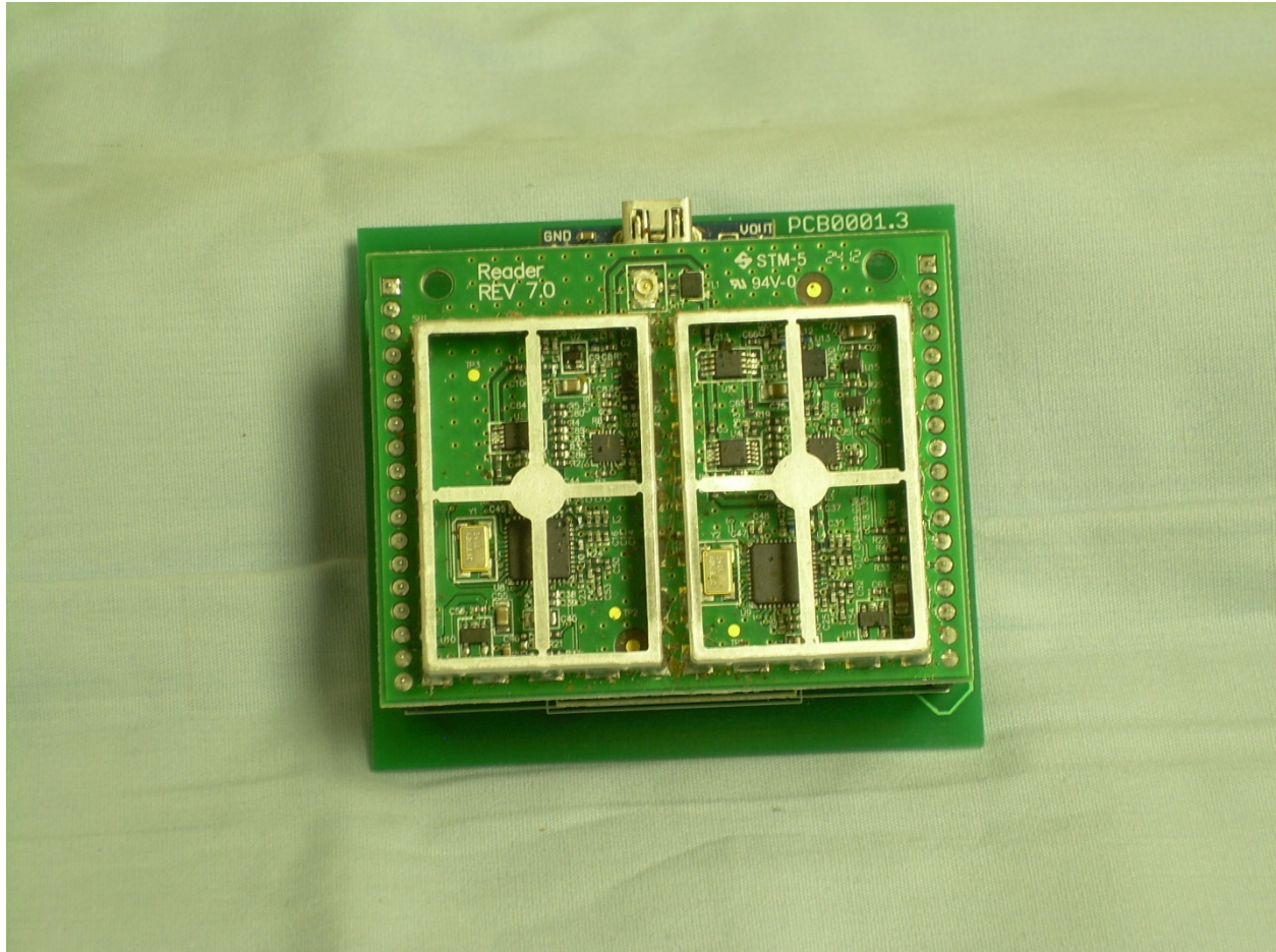
View of the Component Side of the EUT RF PCB with RF Shield Tops Removed
