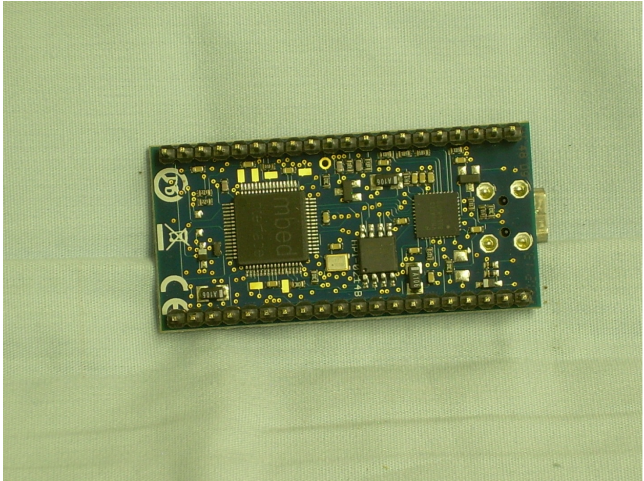
View of the Bottom Side of the System Interface PCB
