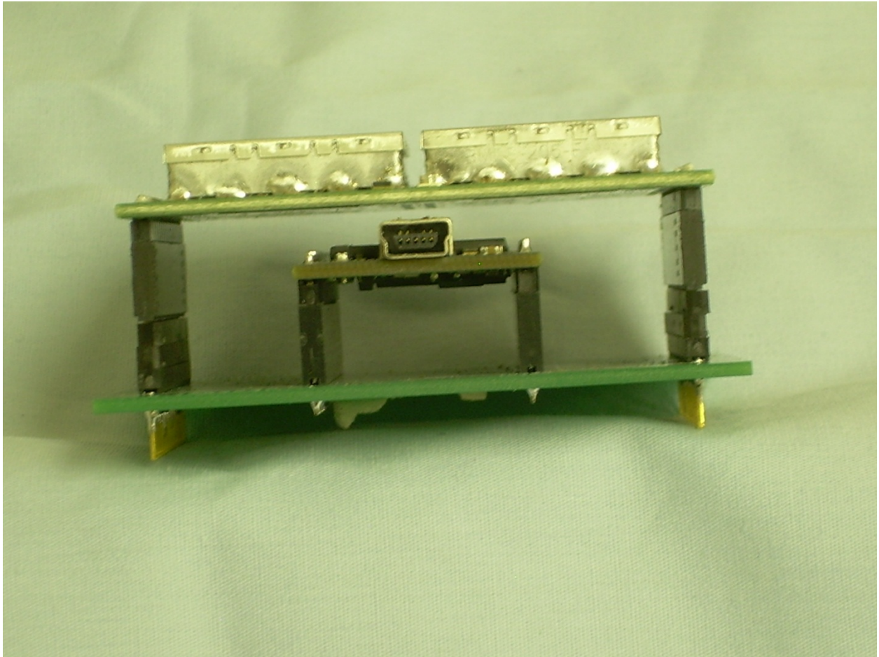
Side View of the EUT
