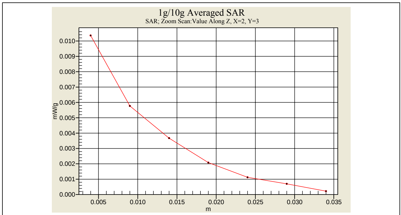
SAR Measurement _ Flat CH4 _Belt-clip
