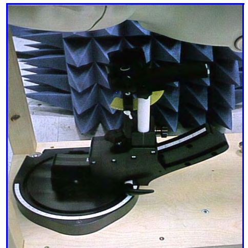
Figure 10. Device Holder
