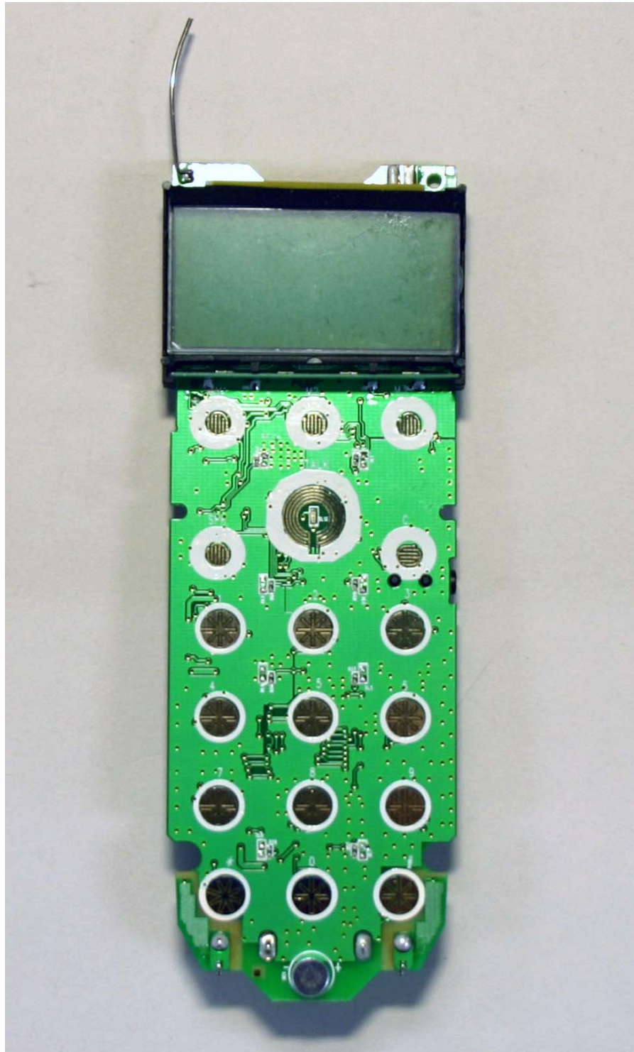
Bottom View
