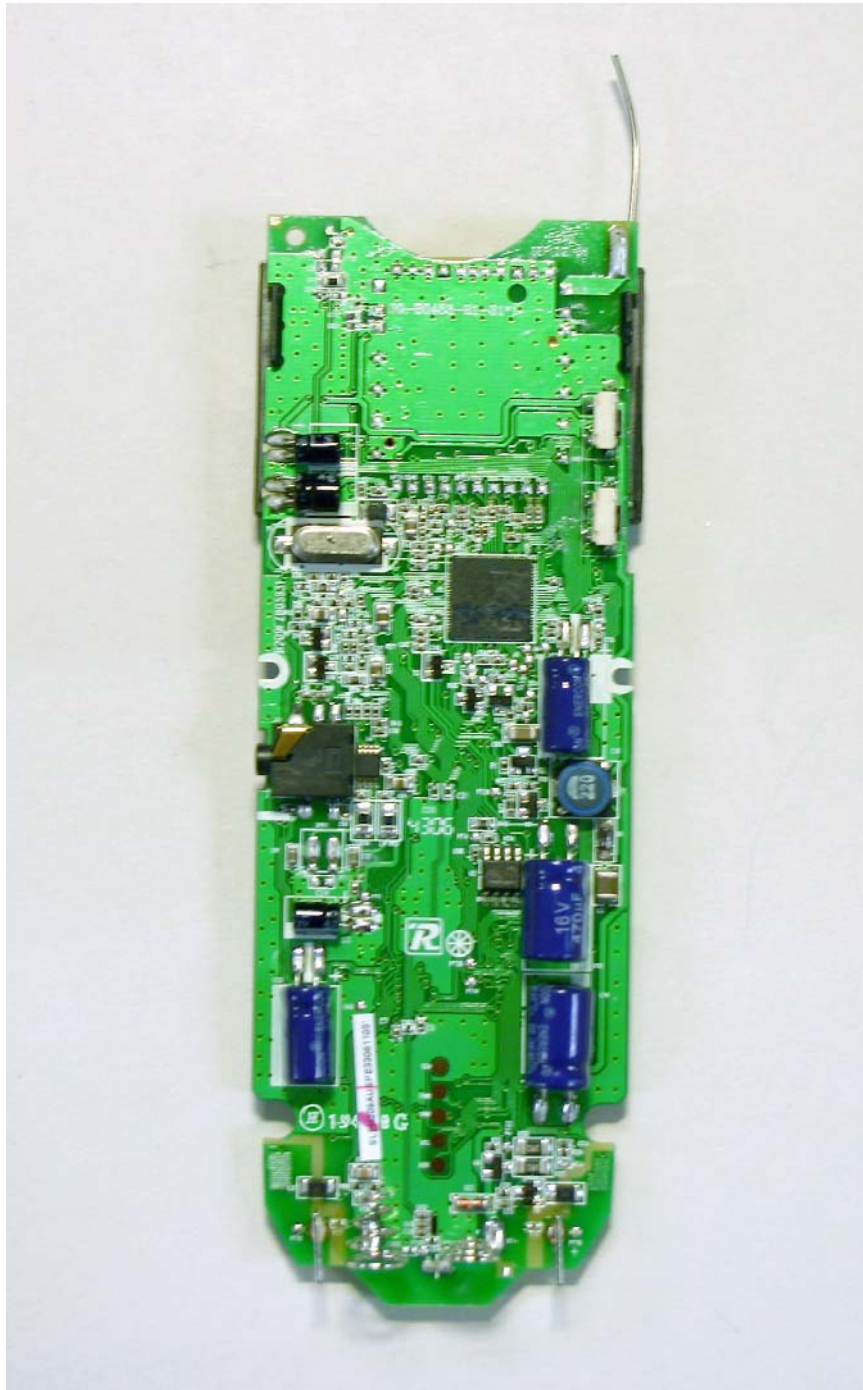
Top View
