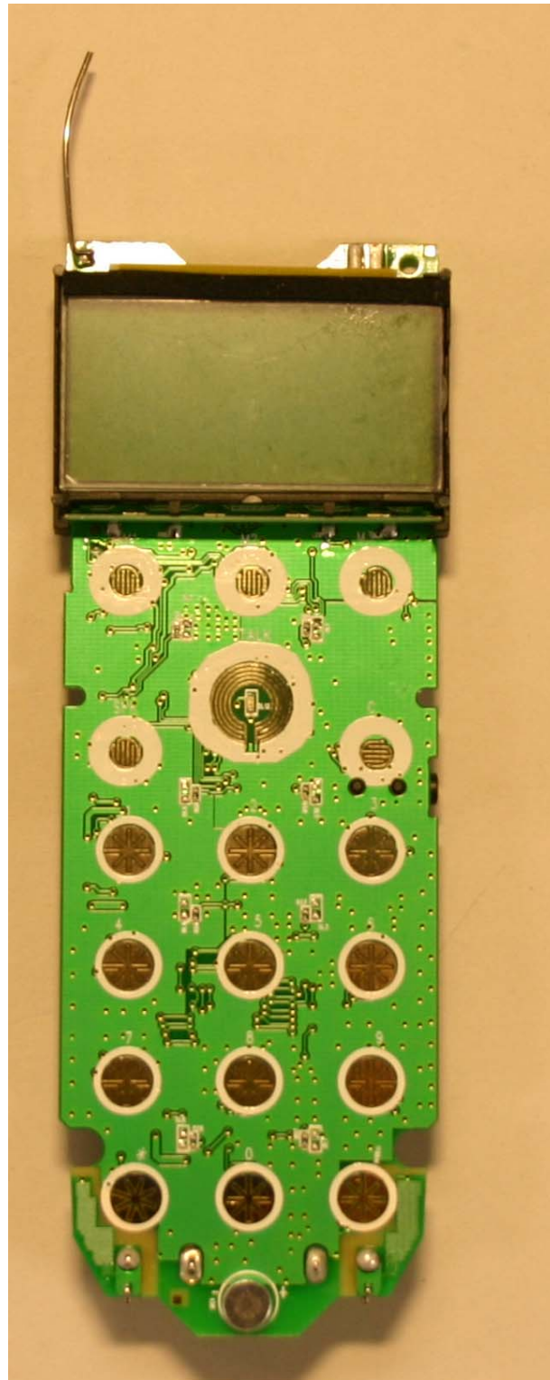
Bottom View
