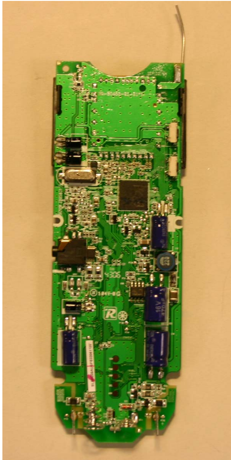
Top View
