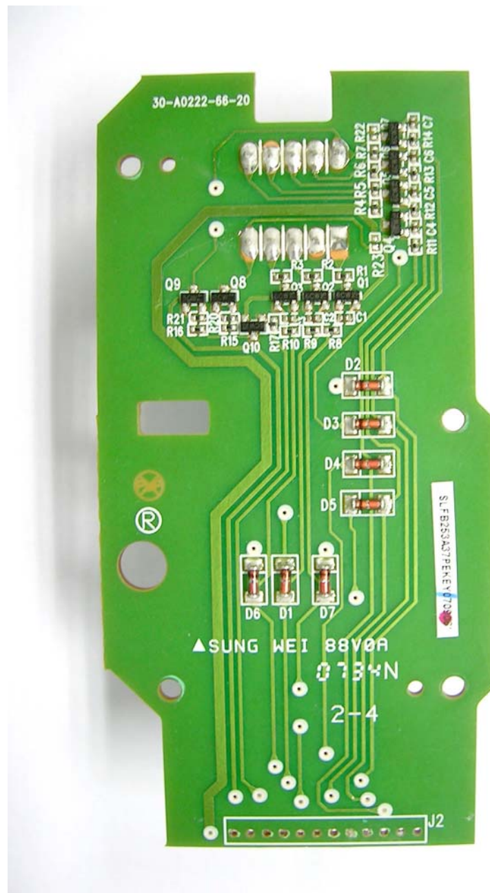
Bottom View
