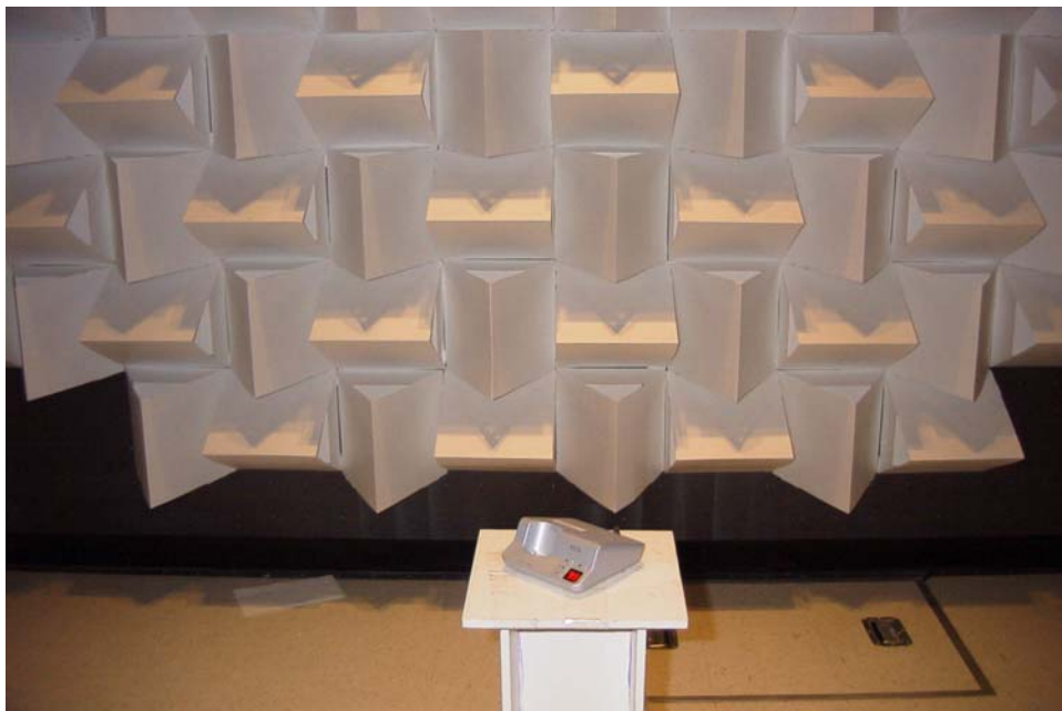
Radiated Test Set Up (Base On Pedestal Table)
