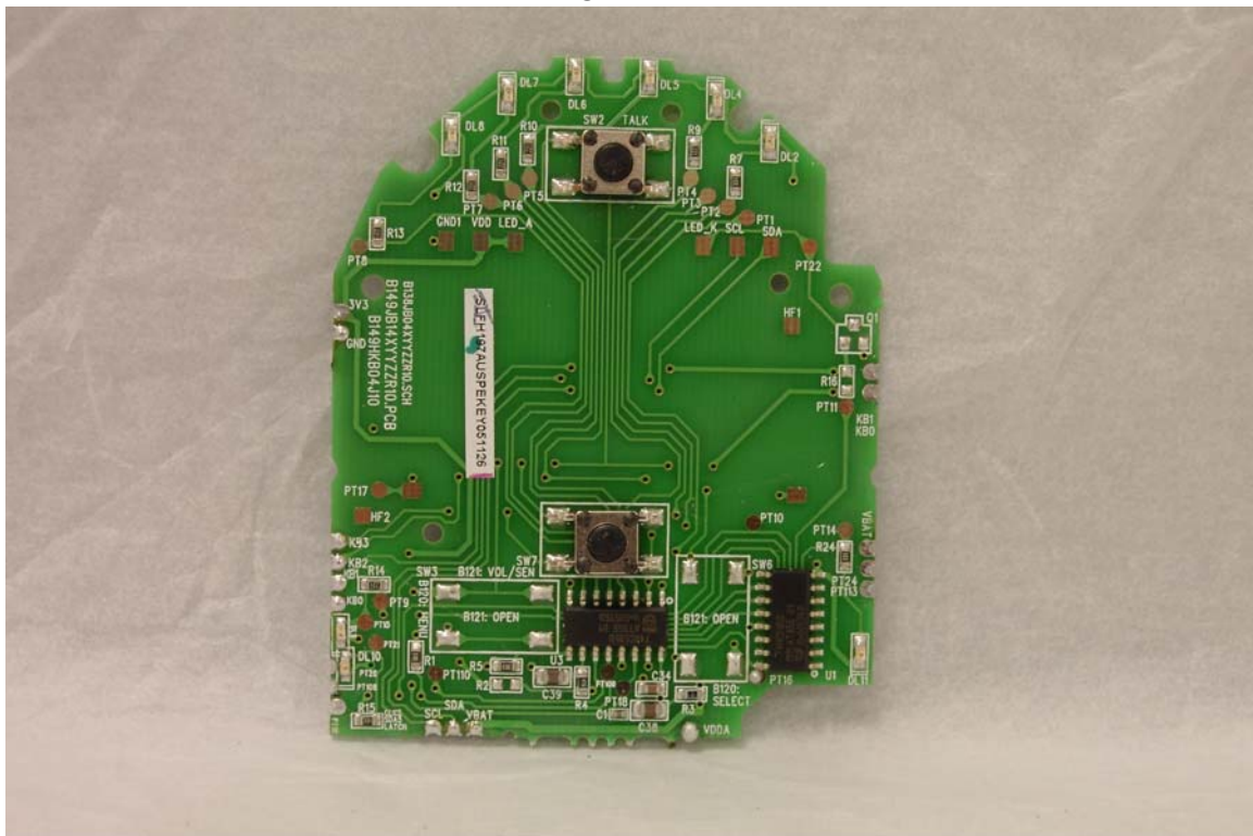
TOP VIEW
