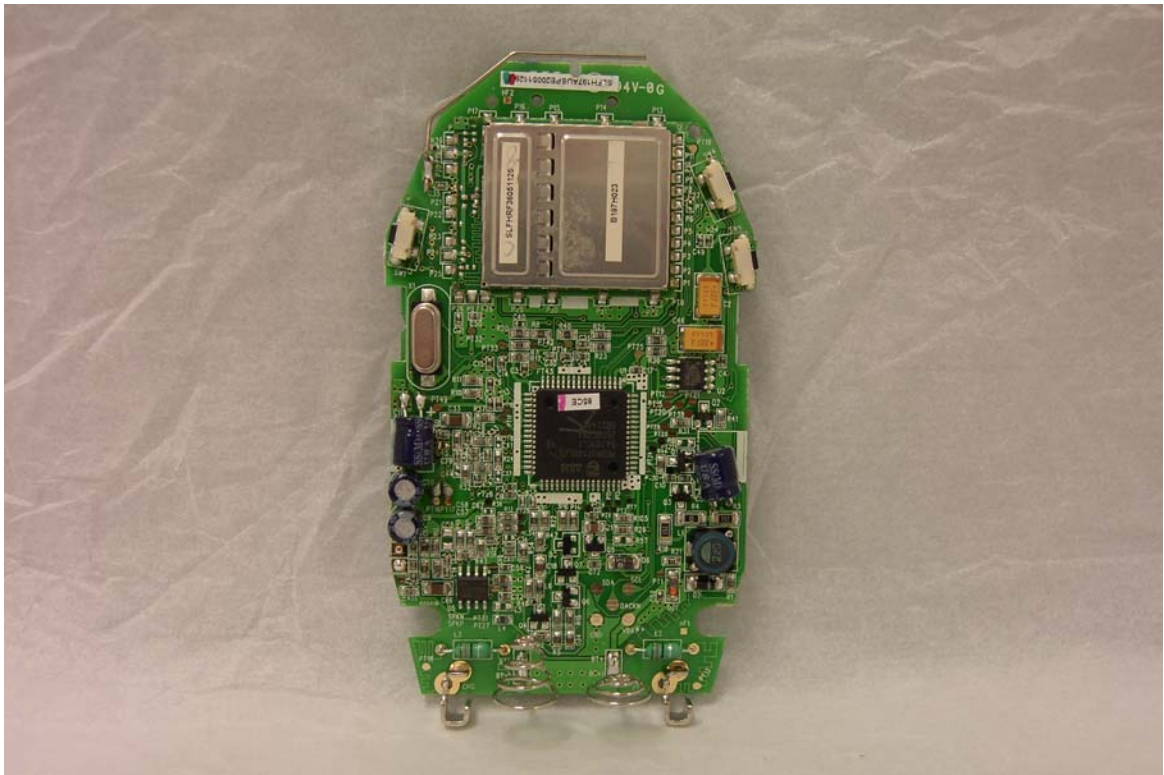
TOP VIEW 1
