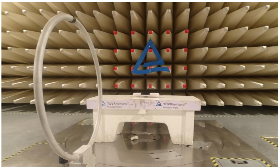
Photo 2: Loop antenna with Perpendicular polarization
