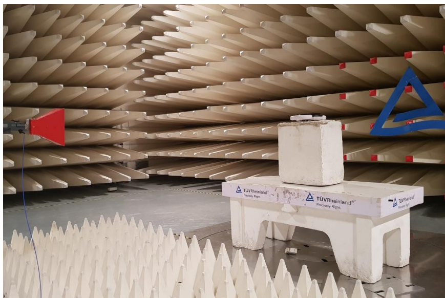
Photo 8: Horn antenna with horizontal polarization
