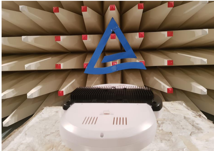
Photo 11: EUT setup
