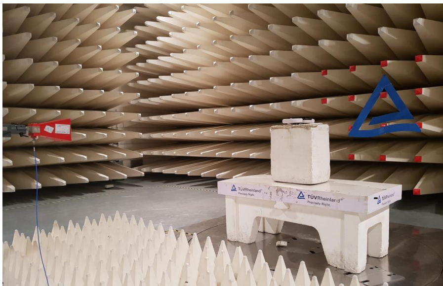
Photo 7: Horn antenna with vertical polarization
