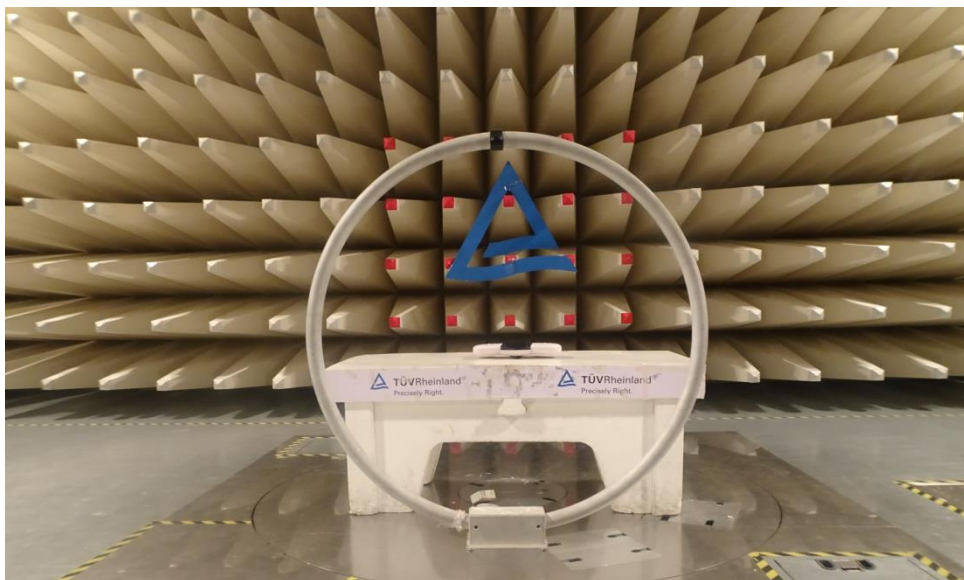
Photo 1 : Loop antenna with Parallel polarization
