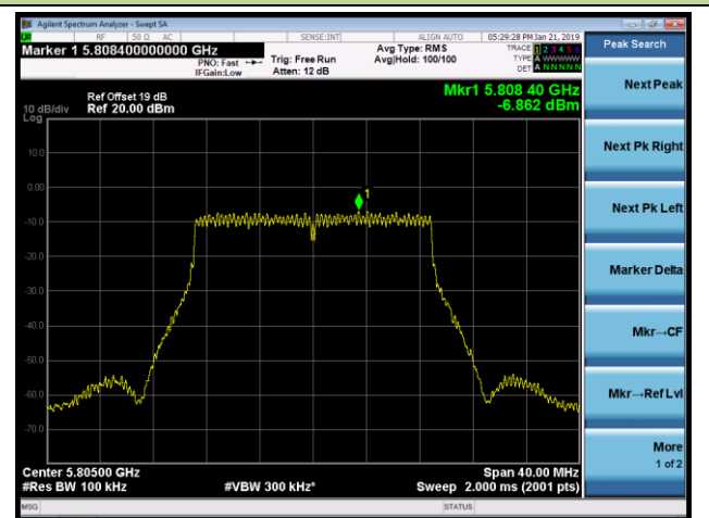
Channel 161 (5805MHz)
