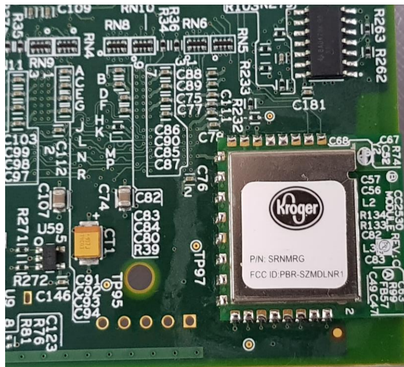
Photo 7: ZigBee Module
