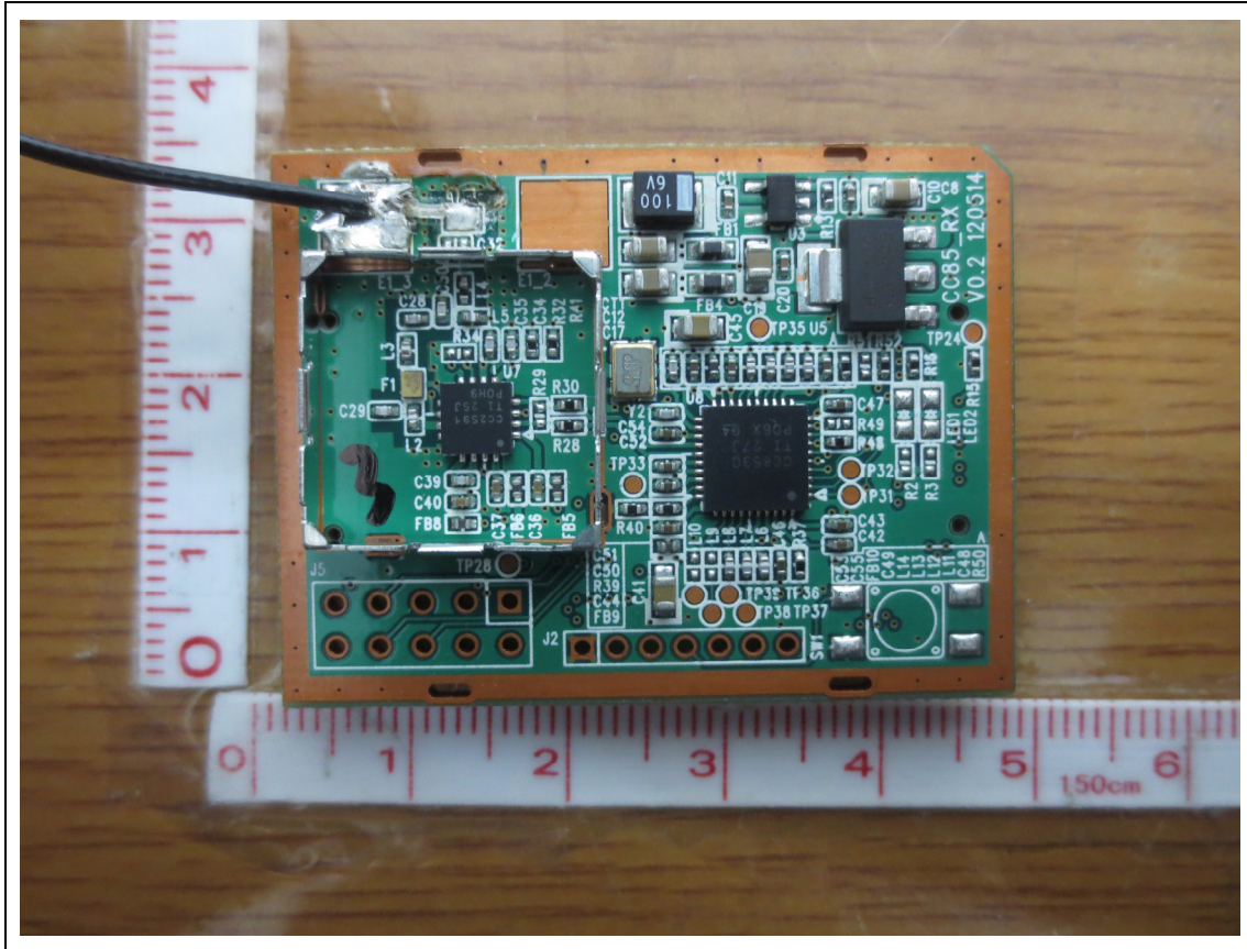
RF Modul Board - Rear
