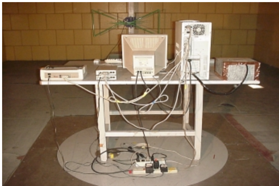
BACK OF RADIATED EMISSION TEST
