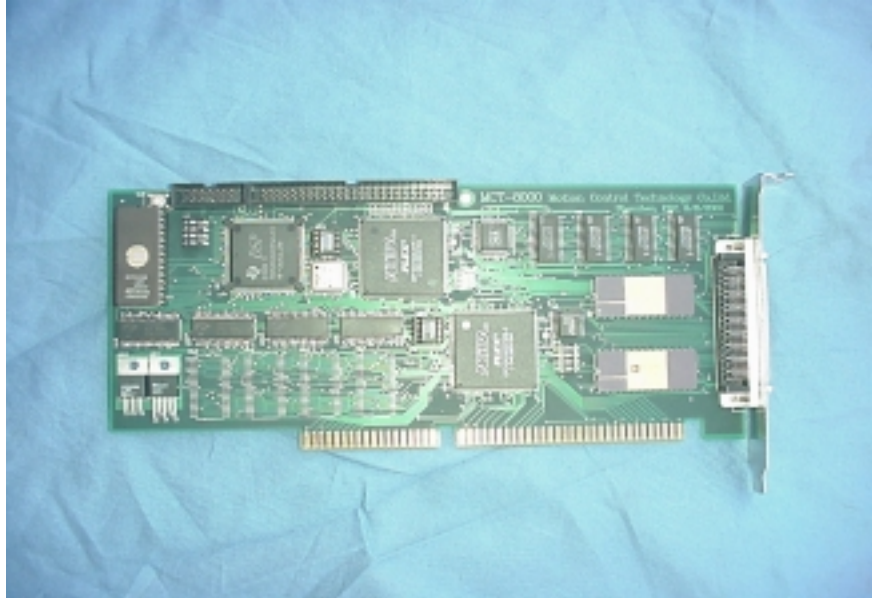
General Appearance of EUT, (Rear View)
