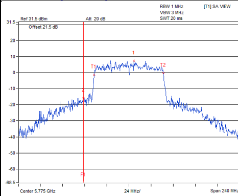
802.11ac(VHT80)_Chain0 / CH155
