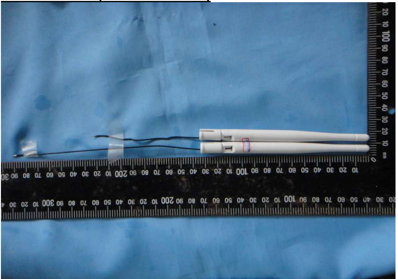
External Photo (Antenna 2.35dBi)
