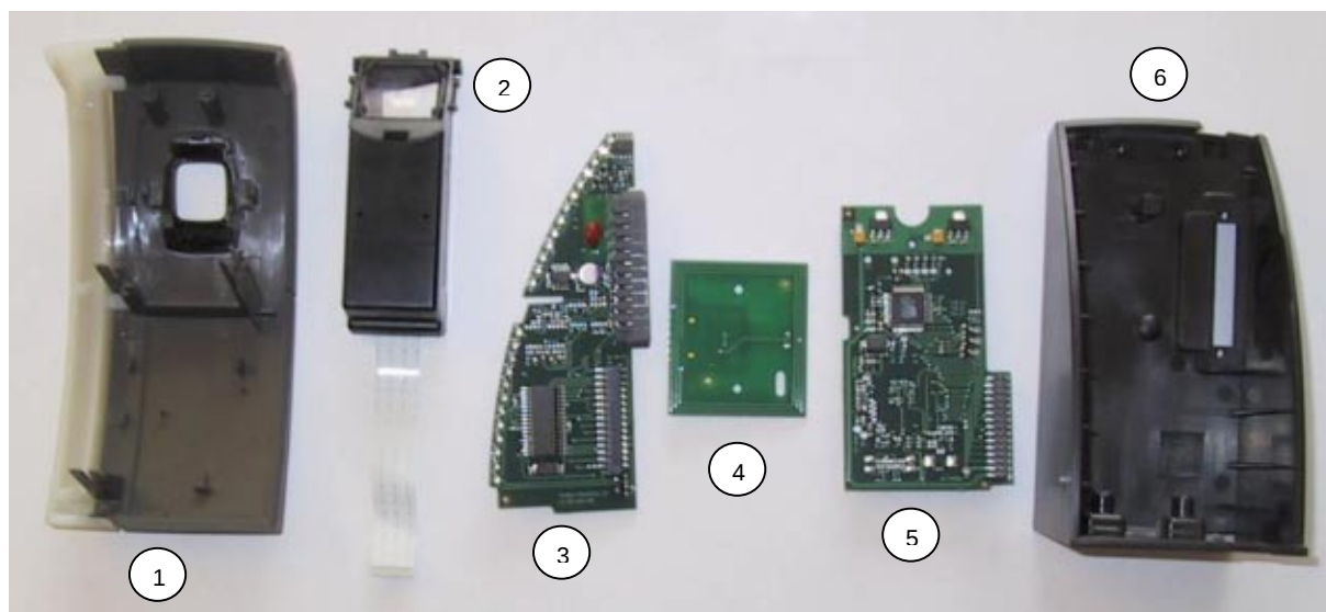
The different parts of the Precise BioAccess Mifare reader
