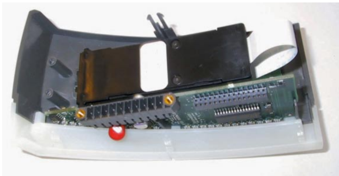
Precise BioAccess Mifare front cover with I/O PCA and fingerprint sensor
