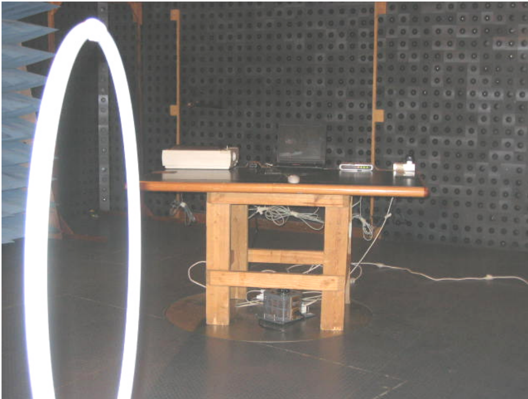
Photograph No.3 Setup for spurious emission field strength measurements in 9 kHz to 30 MHz range
