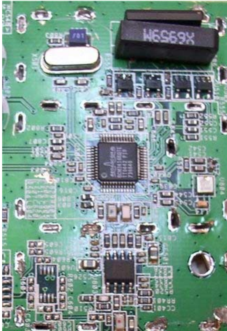
Photograph No.6 RF part with shields removed
