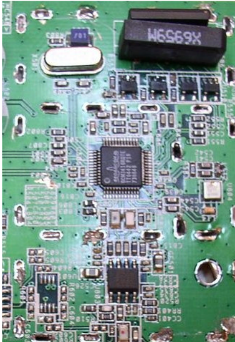
Photograph No.6 RF part with shields removed
