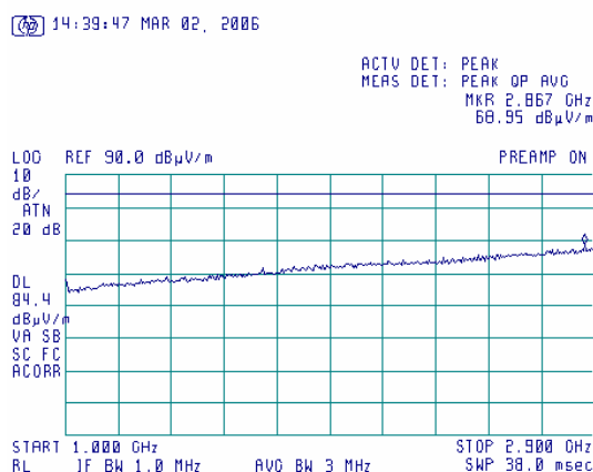
Plot 7.5.20 Radiated emission measurements in 1 – 2.9 GHz range
