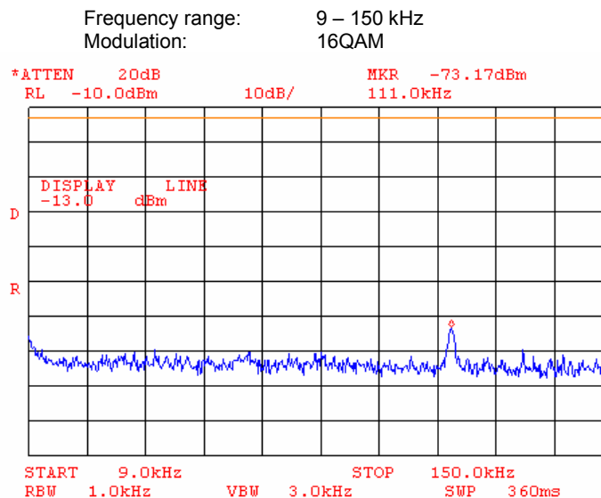
Plot 7.3.3 Spurious emission measurements at RF antenna connector, high channel
