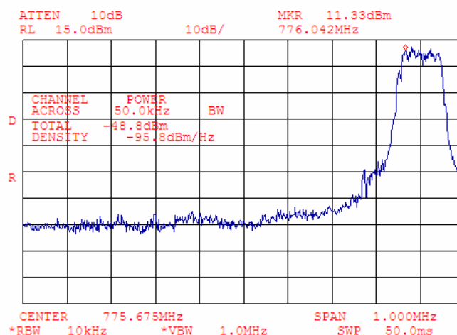
Plot 7.4.48 Adjacent channel coupled power measurements, low carrier frequency
