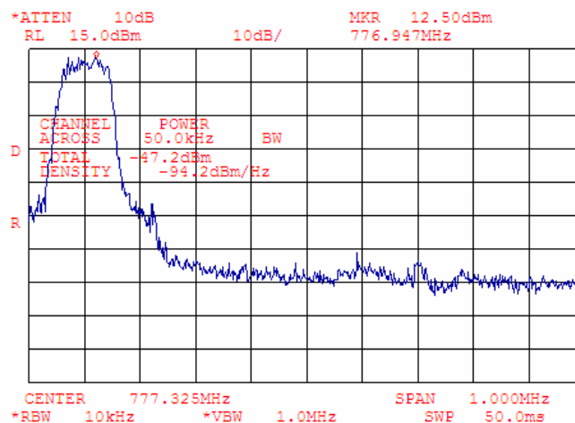
Plot 7.4.35 Adjacent channel coupled power measurements, high carrier frequency
