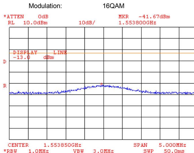
Plot 7.3.17 Spurious emission measurements at RF antenna connector, the 2 nd harmonic of the high channel
