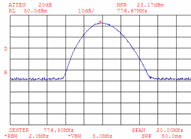
Plot 7.4.66 Adjacent channel coupled power measurements High carrier frequency (776.925 MHz) peak output power: 23.17 dBm
