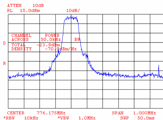
Plot 7.4.2 Adjacent channel coupled power measurements, low carrier frequency
