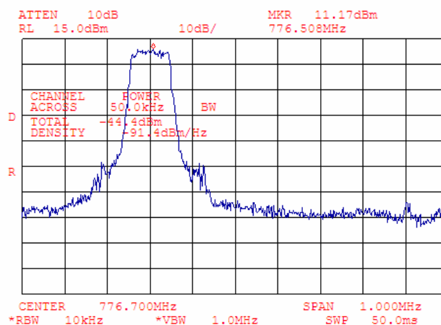
Plot 7.4.56 Adjacent channel coupled power measurements, mid carrier frequency
