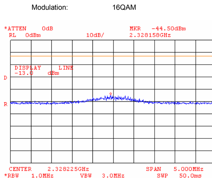
Plot 7.3.14 Spurious emission measurements at RF antenna connector, the 3 rd harmonic of the low channel
