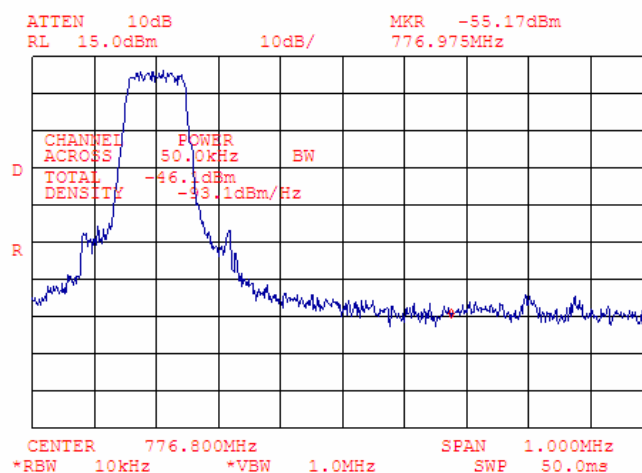
Plot 7.4.58 Adjacent channel coupled power measurements, mid carrier frequency
