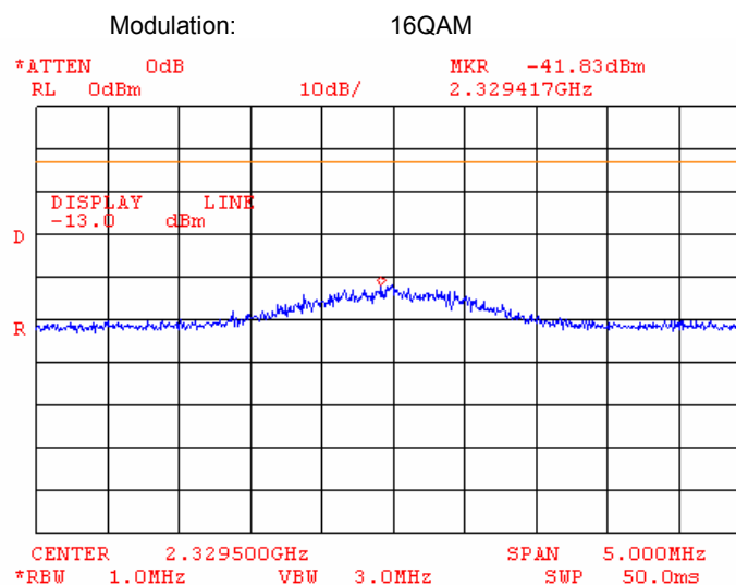
Plot 7.3.16 Spurious emission measurements at RF antenna connector, the 3 rd harmonic of the mid channel
