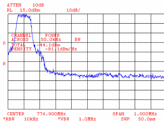
Plot 7.4.22 Adjacent channel coupled power measurements, mid carrier frequency
