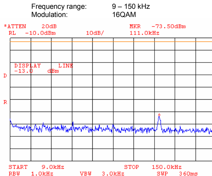
Plot 7.3.1 Spurious emission measurements at RF antenna connector, low channel
