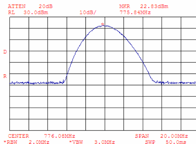
Plot 7.4.40 Adjacent channel coupled power measurements Low carrier frequency (776.075 MHz) peak output power: 22.83 dBm
