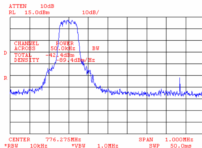
Plot 7.4.5 Adjacent channel coupled power measurements, low carrier frequency
