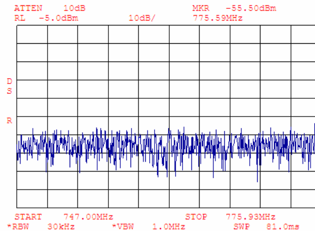
Plot 7.4.77 Adjacent channel coupled power measurements, high carrier frequency
