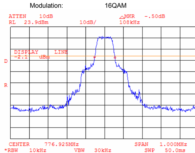
Plot 7.7.6 Occupied bandwidth test results at high frequency
