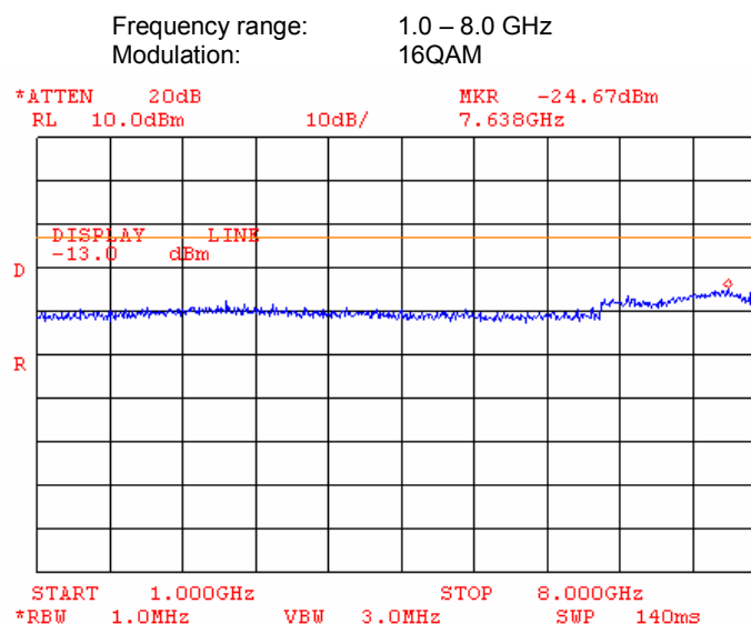
Plot 7.3.11 Spurious emission measurements at RF antenna connector, mid channel
