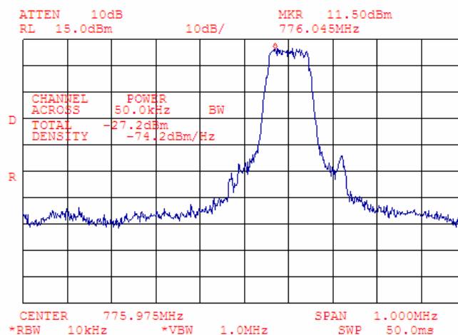
Plot 7.4.42 Adjacent channel coupled power measurements, low carrier frequency
