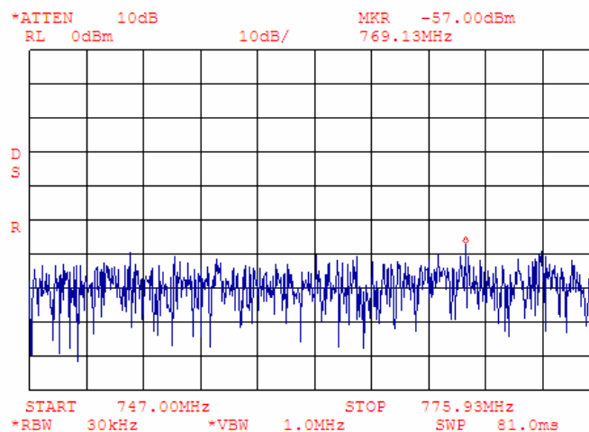
Plot 7.4.39 Adjacent channel coupled power measurements, high carrier frequency
