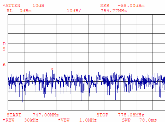
Plot 7.4.13 Adjacent channel coupled power measurements, low carrier frequency
