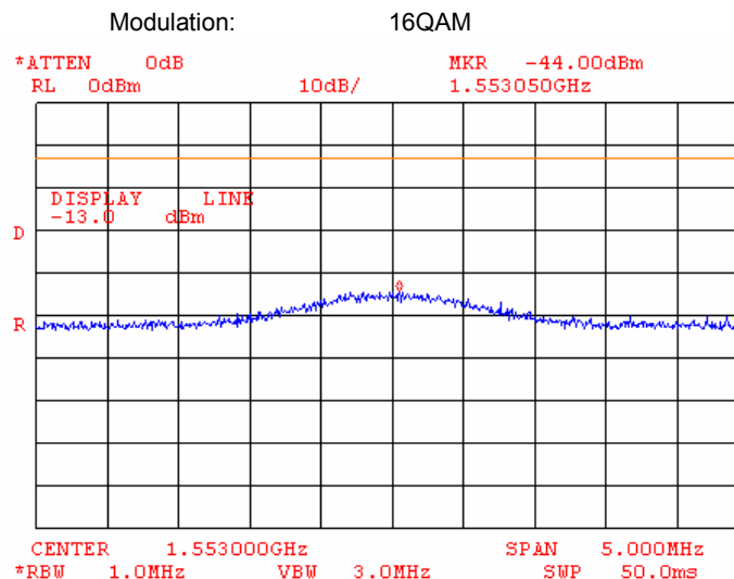
Plot 7.3.15 Spurious emission measurements at RF antenna connector, the 2 nd harmonic of the mid channel
