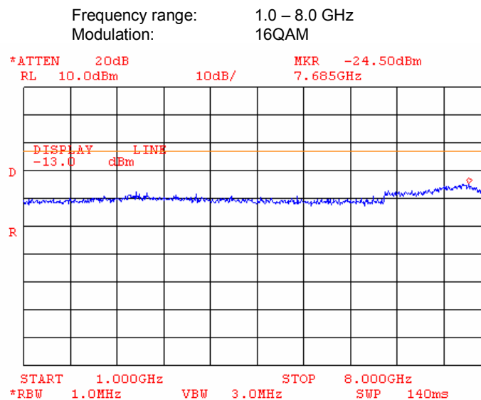
Plot 7.3.12 Spurious emission measurements at RF antenna connector, high channel
