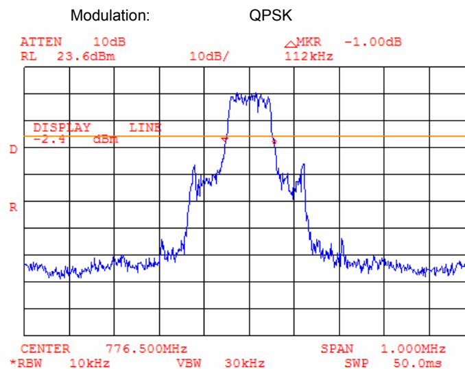
Plot 7.7.2 Occupied bandwidth test results at mid frequency
