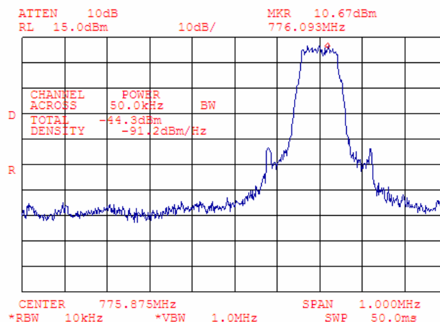
Plot 7.4.44 Adjacent channel coupled power measurements, low carrier frequency
