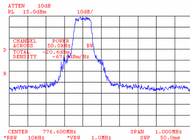
Plot 7.4.16 Adjacent channel coupled power measurements, mid carrier frequency
