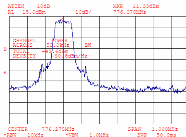
Plot 7.4.43 Adjacent channel coupled power measurements, low carrier frequency
