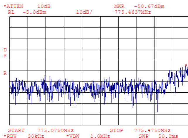
Plot 7.4.50 Adjacent channel coupled power measurements, low carrier frequency
