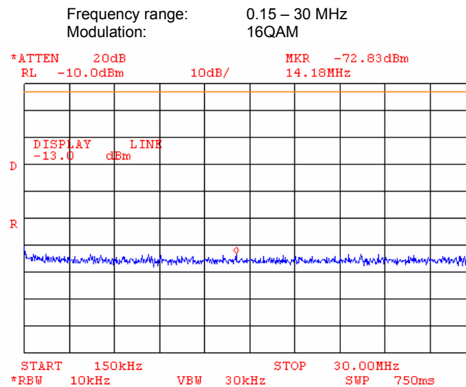
Plot 7.3.6 Spurious emission measurements at RF antenna connector, high channel
