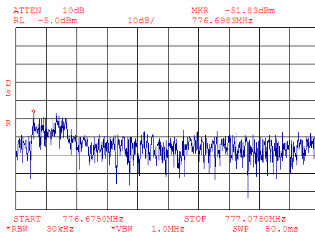
Plot 7.4.49 Adjacent channel coupled power measurements, low carrier frequency
