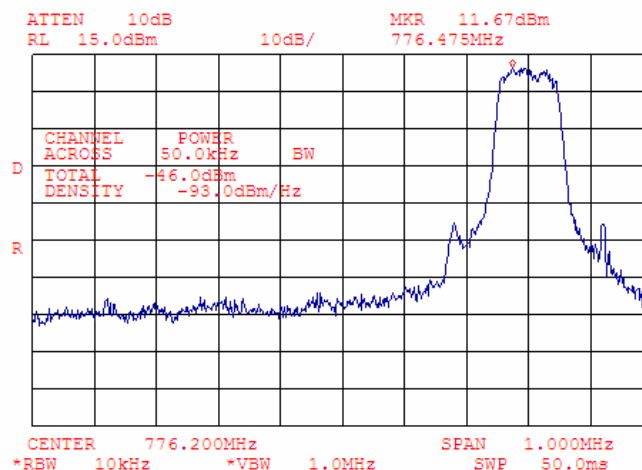
Plot 7.4.59 Adjacent channel coupled power measurements, mid carrier frequency
