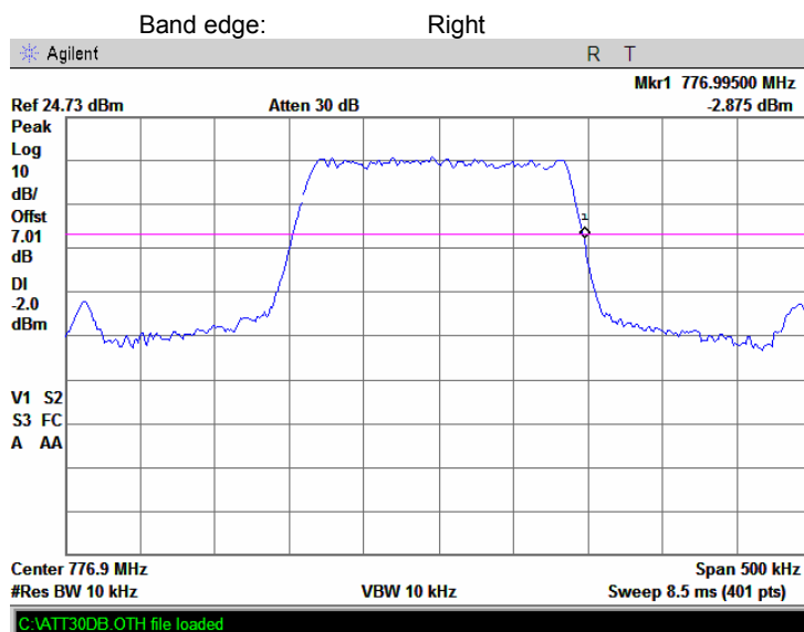
Plot 7.6.2 Band edge emission at high frequency
