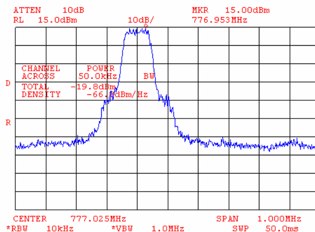
Plot 7.4.29 Adjacent channel coupled power measurements, high carrier frequency
