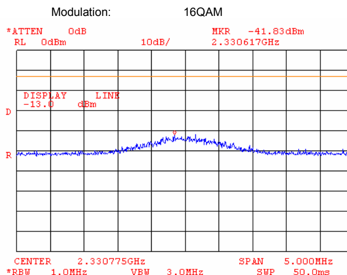
Plot 7.3.18 Spurious emission measurements at RF antenna connector, the 3 rd harmonic of the high channel
