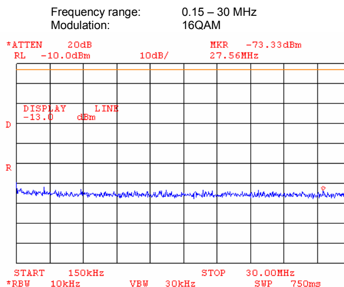
Plot 7.3.4 Spurious emission measurements at RF antenna connector, low channel
