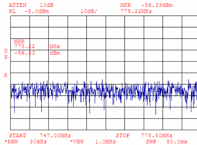
Plot 7.4.65 Adjacent channel coupled power measurements, mid carrier frequency
