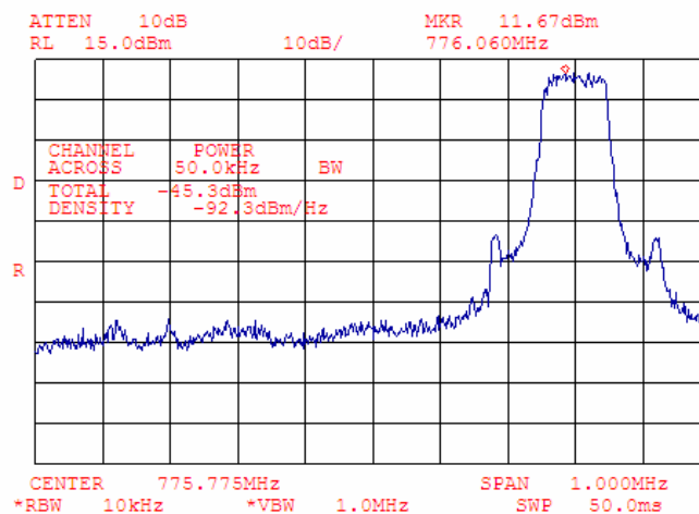
Plot 7.4.46 Adjacent channel coupled power measurements, low carrier frequency
