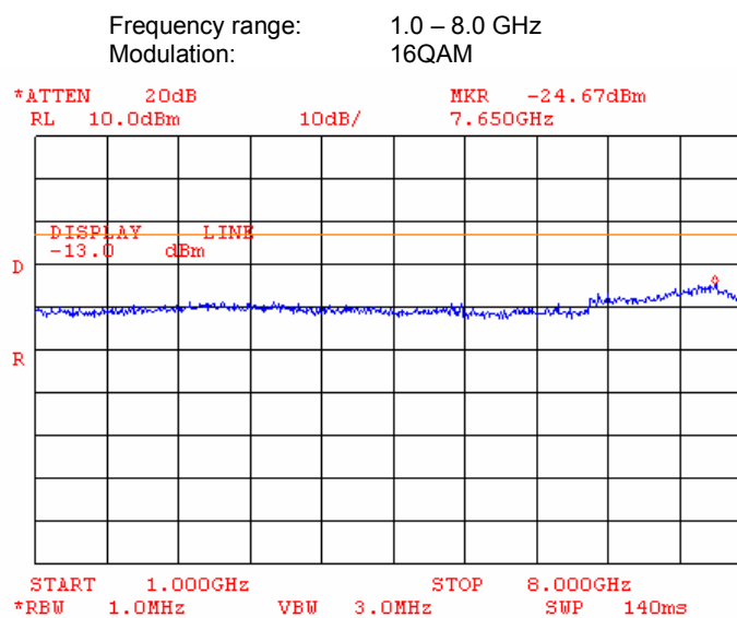
Plot 7.3.10 Spurious emission measurements at RF antenna connector, low channel
