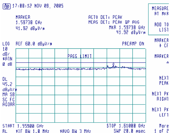
Plot 7.8.2 Radiated emission measurements in 1559 - 1610 MHz range
