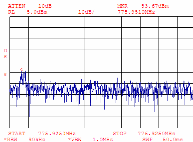
Plot 7.4.76 Adjacent channel coupled power measurements, high carrier frequency
