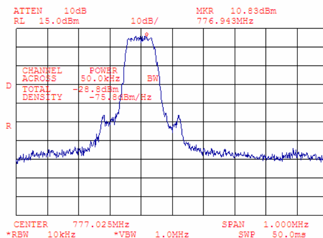
Plot 7.4.67 Adjacent channel coupled power measurements, high carrier frequency
