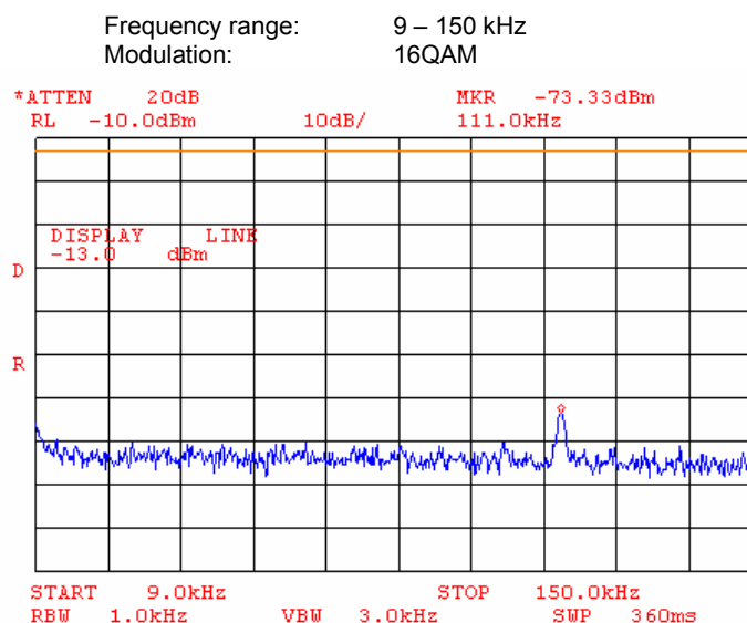
Plot 7.3.2 Spurious emission measurements at RF antenna connector, mid channel
