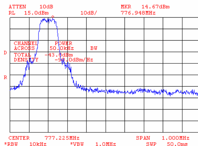
Plot 7.4.33 Adjacent channel coupled power measurements, high carrier frequency
