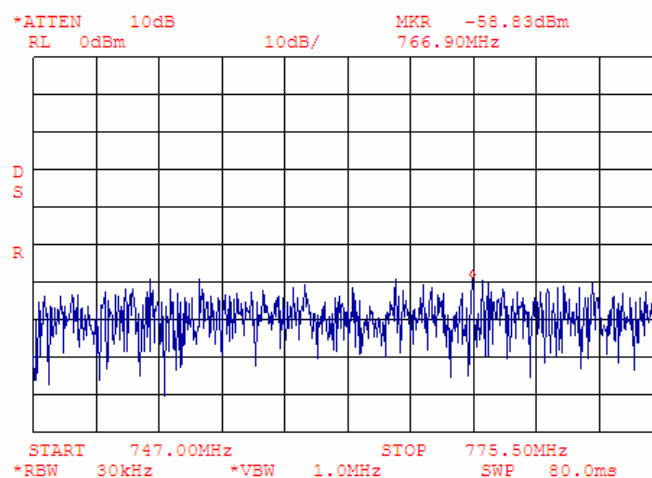
Plot 7.4.26 Adjacent channel coupled power measurements, mid carrier frequency
