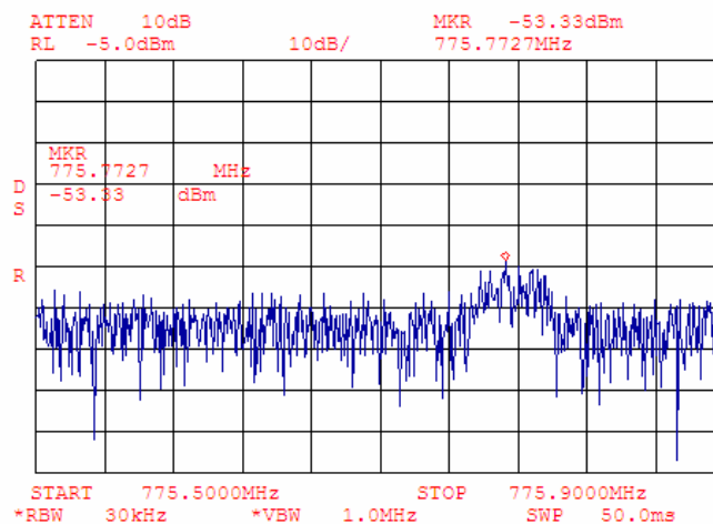
Plot 7.4.63 Adjacent channel coupled power measurements, mid carrier frequency
