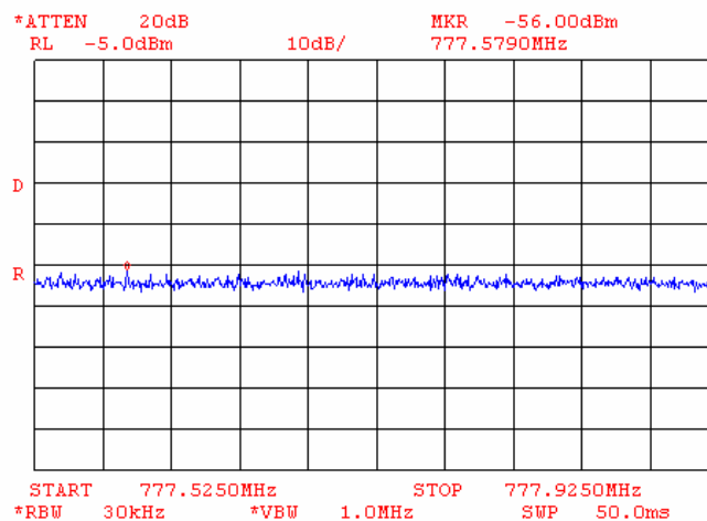
Plot 7.4.37 Adjacent channel coupled power measurements, high carrier frequency
