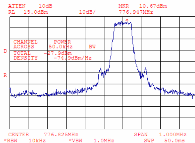
Plot 7.4.68 Adjacent channel coupled power measurements, high carrier frequency
