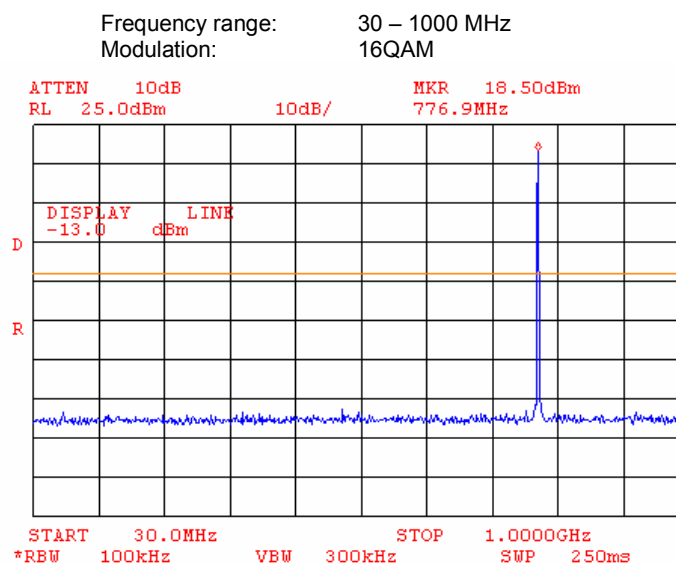
Plot 7.3.8 Spurious emission measurements at RF antenna connector, mid channel
