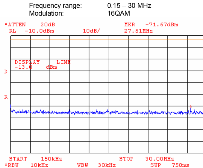
Plot 7.3.5 Spurious emission measurements at RF antenna connector, mid channel
