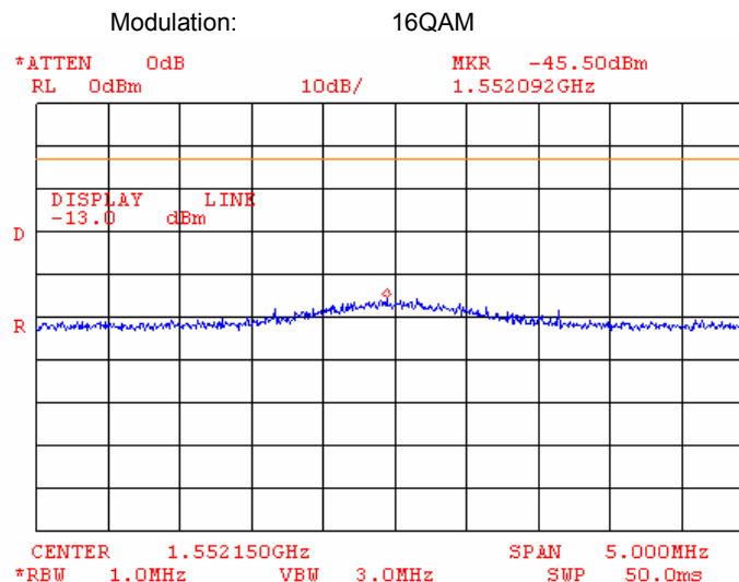
Plot 7.3.13 Spurious emission measurements at RF antenna connector, the 2 nd harmonic of the low channel
