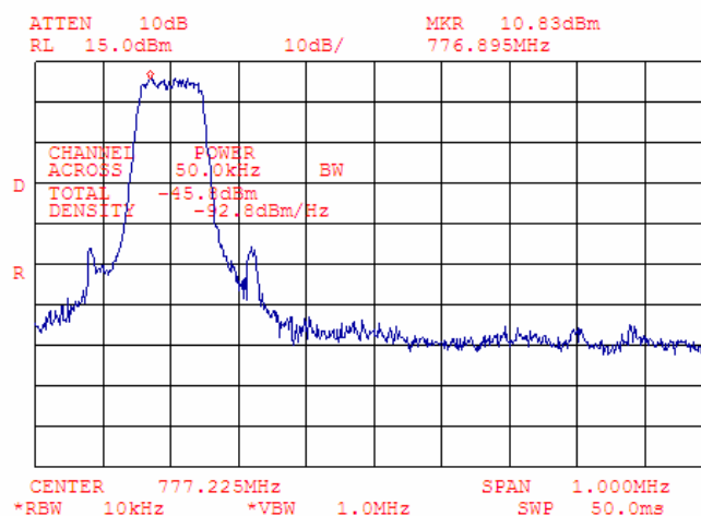
Plot 7.4.71 Adjacent channel coupled power measurements, high carrier frequency
