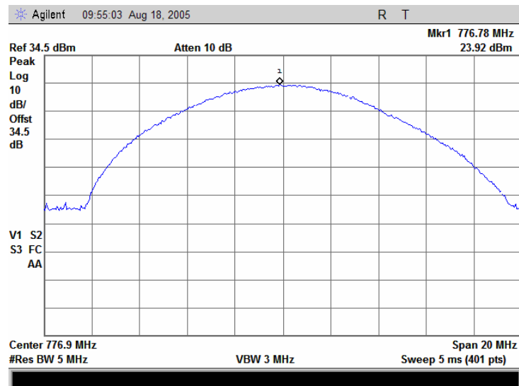
Plot 7.4.27 Adjacent channel coupled power measurements High carrier frequency (776.925 MHz) peak output power: 23.92 dBm
