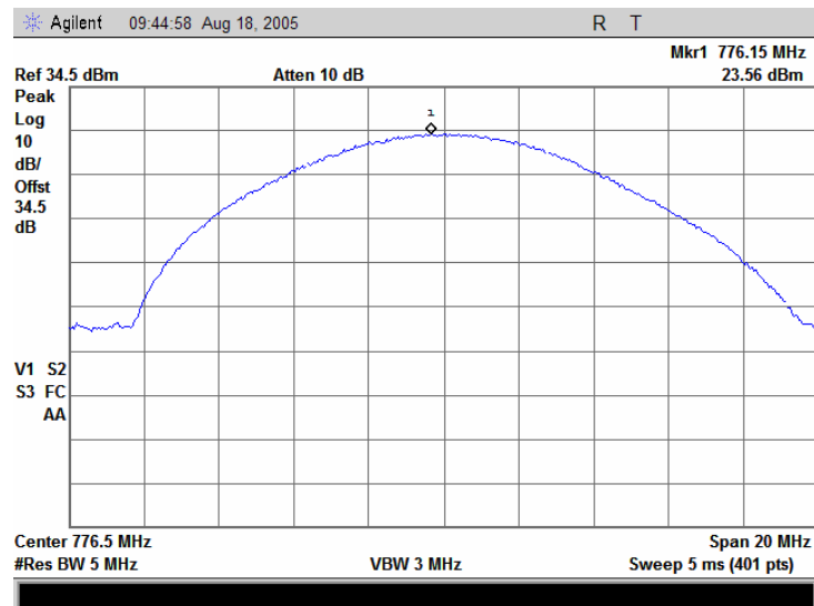
Plot 7.4.14 Adjacent channel coupled power measurements Mid carrier frequency (776.5 MHz) peak output power: 23.56 dBm
