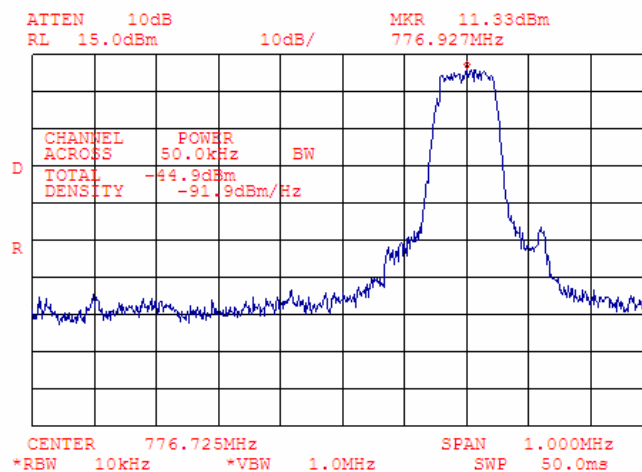
Plot 7.4.70 Adjacent channel coupled power measurements, high carrier frequency
