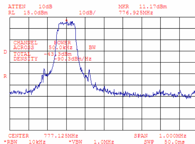
Plot 7.4.69 Adjacent channel coupled power measurements, high carrier frequency
