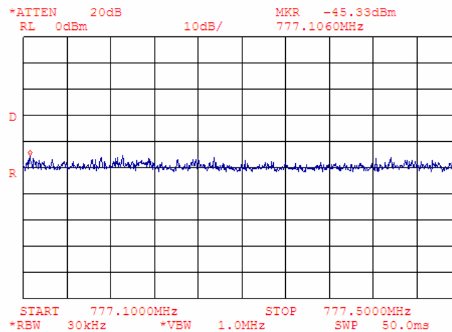
Plot 7.4.24 Adjacent channel coupled power measurements, mid carrier frequency
