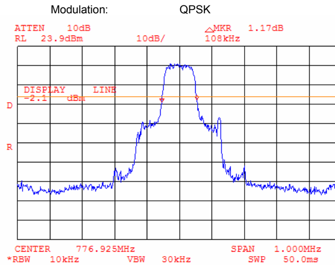
Plot 7.7.3 Occupied bandwidth test results at high frequency
