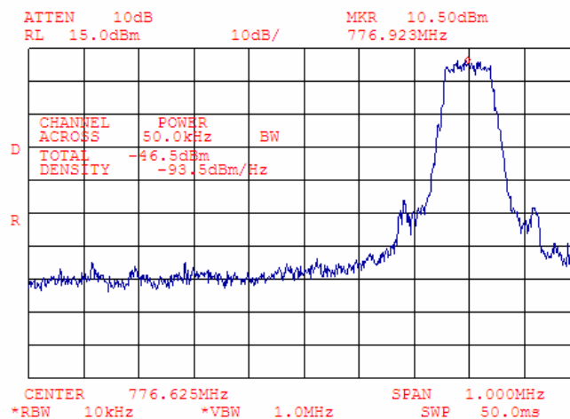
Plot 7.4.72 Adjacent channel coupled power measurements, high carrier frequency
