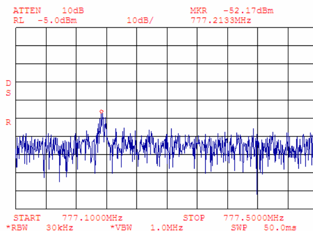
Plot 7.4.62 Adjacent channel coupled power measurements, mid carrier frequency
