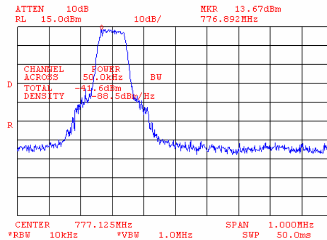
Plot 7.4.31 Adjacent channel coupled power measurements, high carrier frequency
