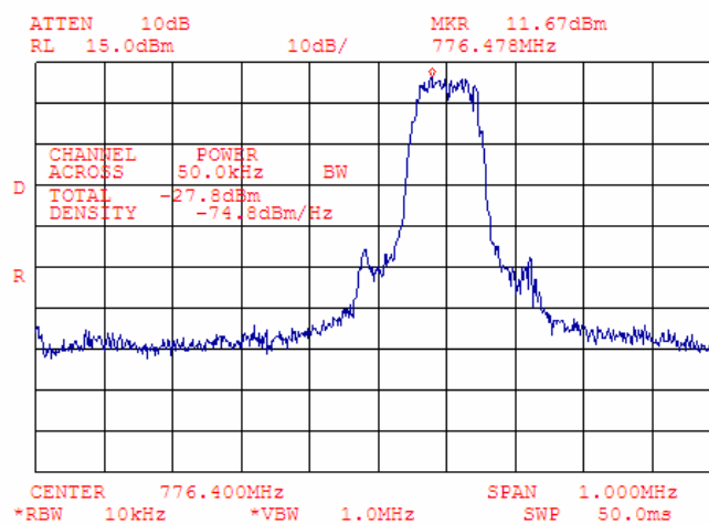
Plot 7.4.55 Adjacent channel coupled power measurements, mid carrier frequency
