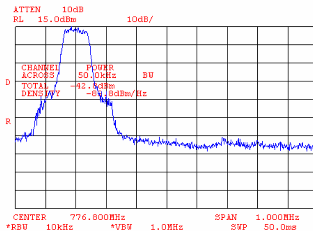
Plot 7.4.20 Adjacent channel coupled power measurements, mid carrier frequency
