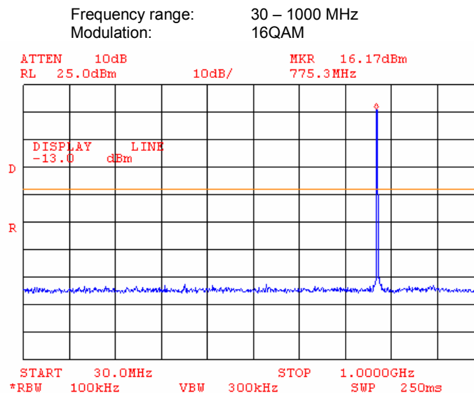
Plot 7.3.7 Spurious emission measurements at RF antenna connector, low channel
