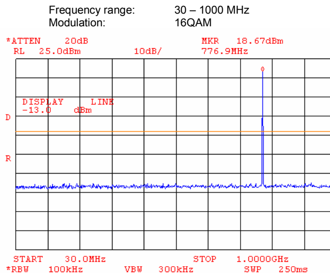
Plot 7.3.9 Spurious emission measurements at RF antenna connector, high channel
