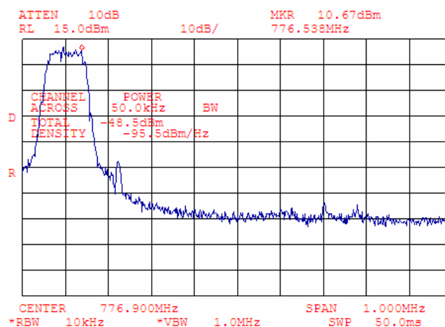
Plot 7.4.60 Adjacent channel coupled power measurements, mid carrier frequency
