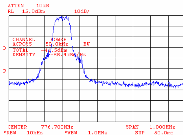
Plot 7.4.18 Adjacent channel coupled power measurements, mid carrier frequency
