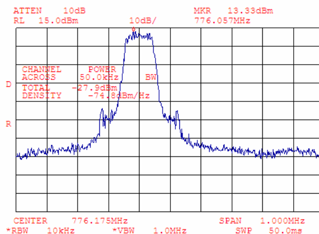
Plot 7.4.41 Adjacent channel coupled power measurements, low carrier frequency
