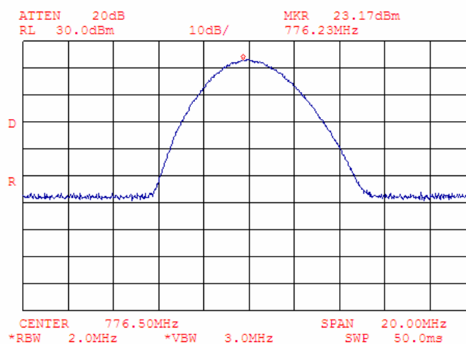
Plot 7.4.53 Adjacent channel coupled power measurements Mid carrier frequency (776.5 MHz) peak output power: 23.17 dBm
