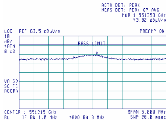
Plot 7.5.20 Radiated emission measurements at the 2 nd harmonic of mid channel
