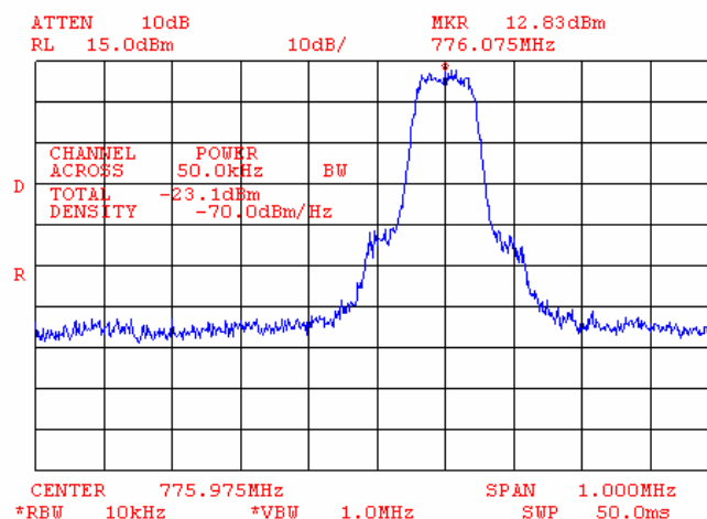
Plot 7.4.3 Adjacent channel coupled power measurements, low carrier frequency
