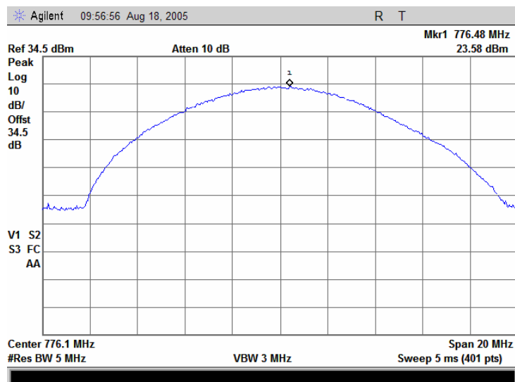
Plot 7.4.1 Adjacent channel coupled power measurements Low carrier frequency (776.075 MHz) peak output power: 23.58 dBm
