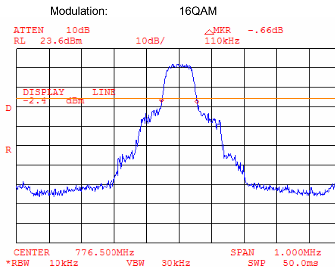
Plot 7.7.5 Occupied bandwidth test results at mid frequency
