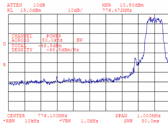
Plot 7.4.61 Adjacent channel coupled power measurements, mid carrier frequency
