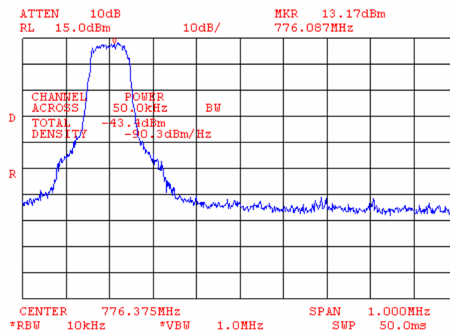
Plot 7.4.7 Adjacent channel coupled power measurements, low carrier frequency
