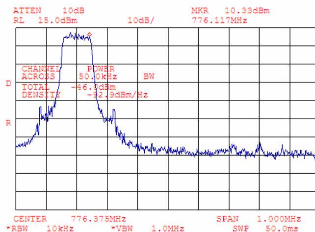
Plot 7.4.45 Adjacent channel coupled power measurements, low carrier frequency
