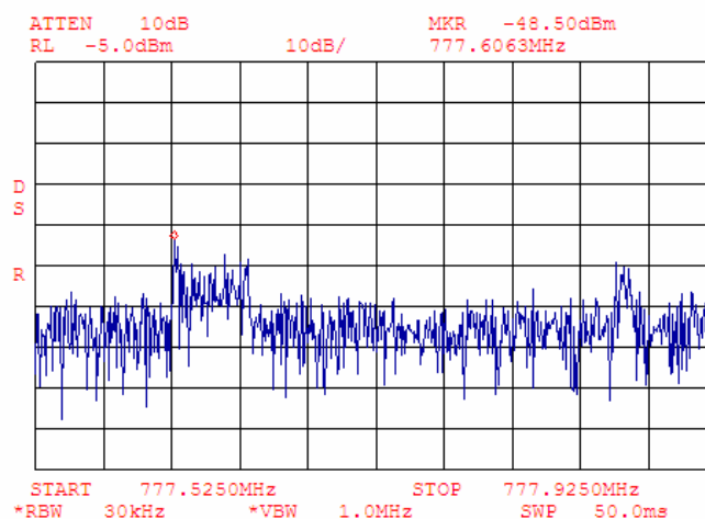
Plot 7.4.75 Adjacent channel coupled power measurements, high carrier frequency
