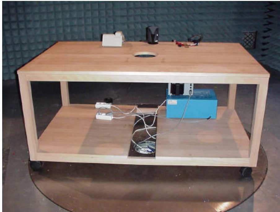
Picture 3 : Setup for radiated measurements, front view
