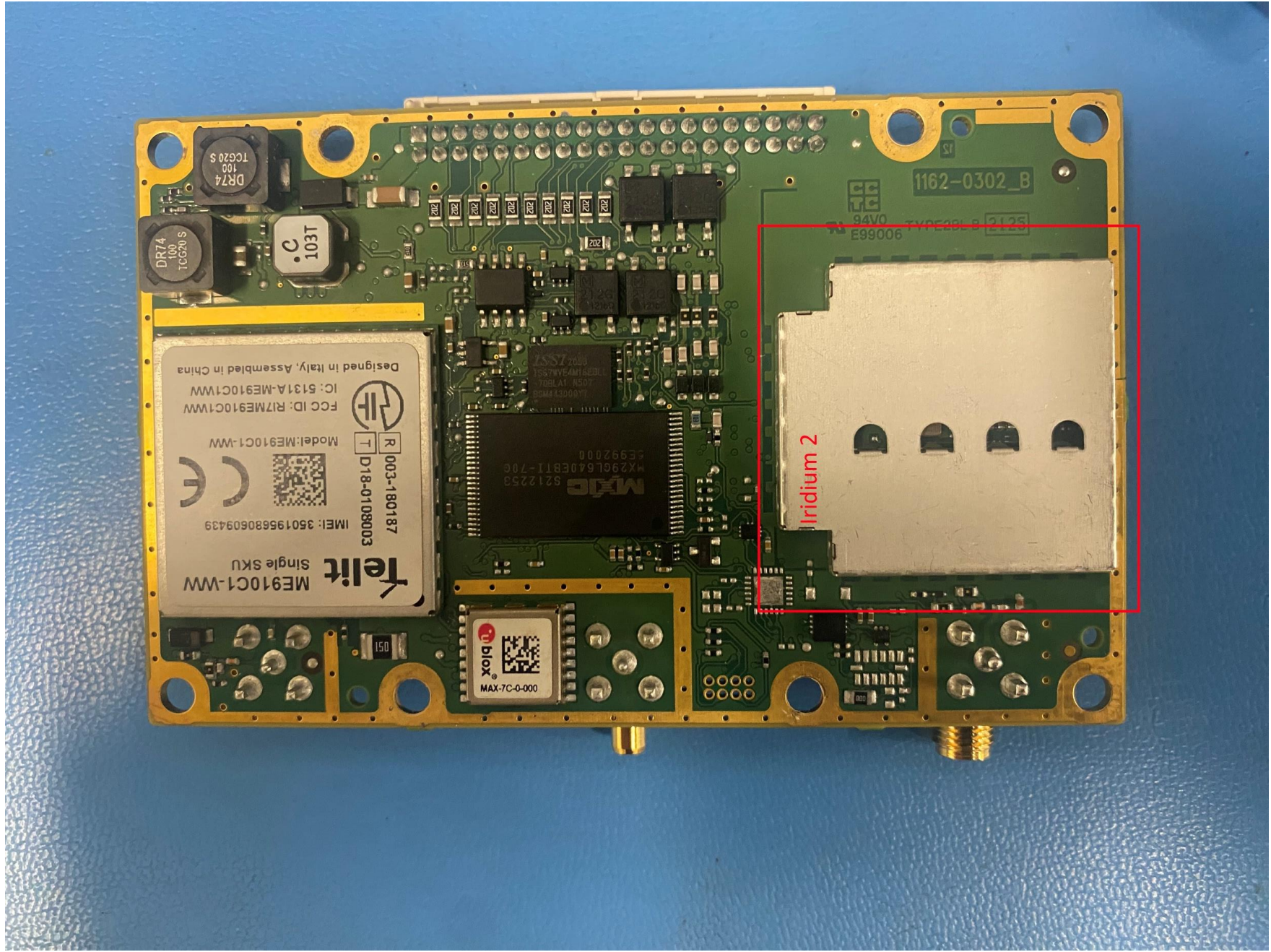
PICTURE 1: Q4000 Back View
