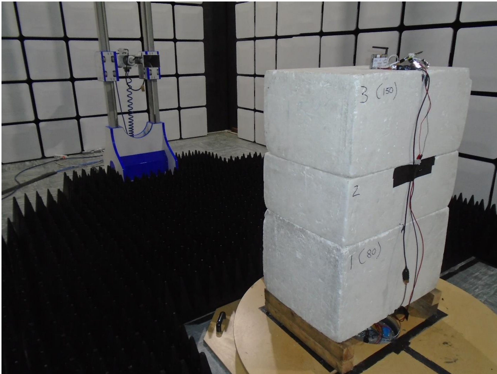
Picture 2: 1 GHz – 18 GHz Test
