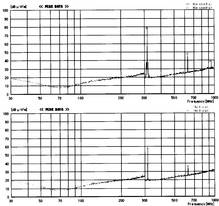
Figure 5. 30-1000MHz spectrum chart
