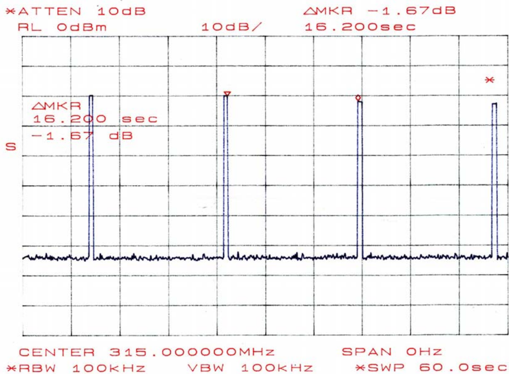
Figure 4. Transmission interval
