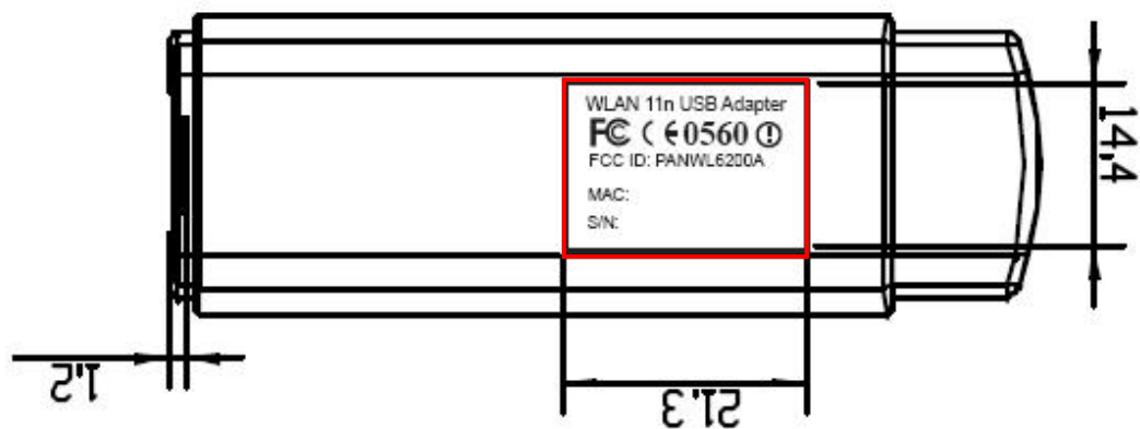
Label Location
