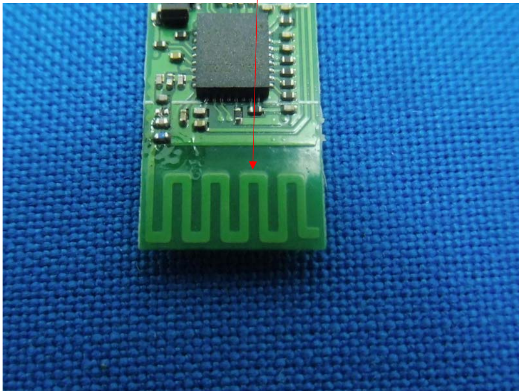
Printed Antenna
