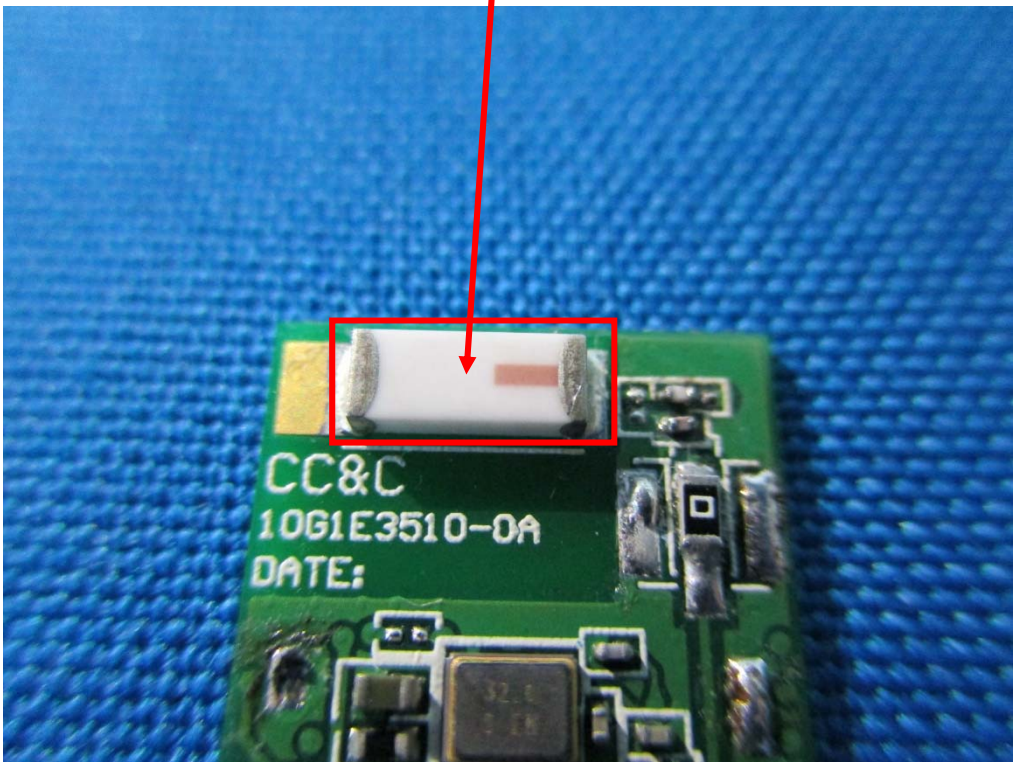
Chip Antenna View
