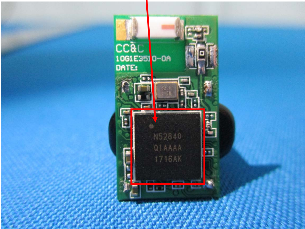
Bluetooth LE IC – Top View
