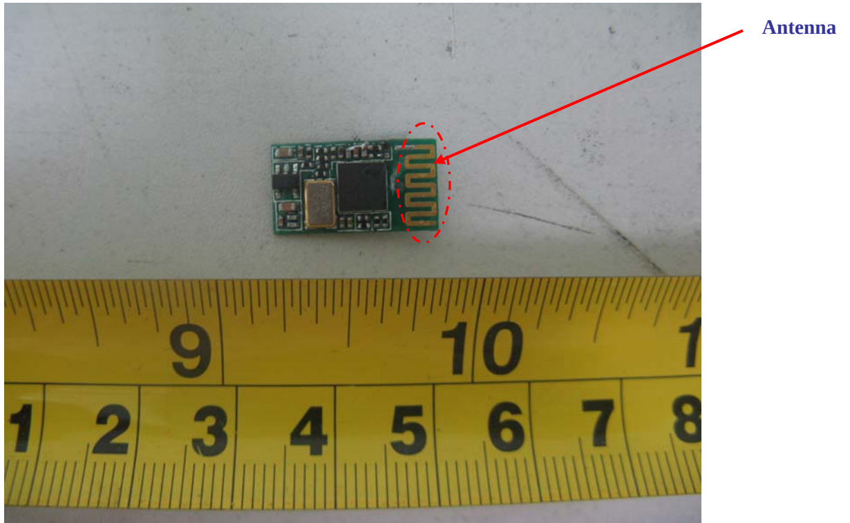
EUT – Controlboard Top Components View
