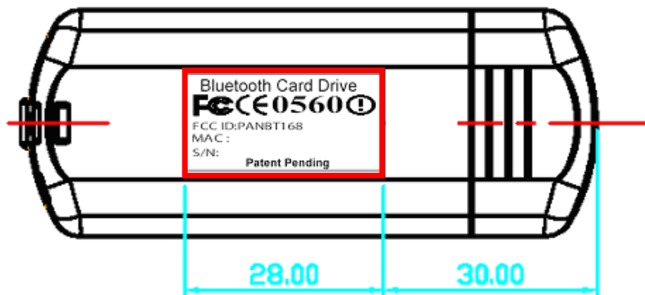
Label Position
