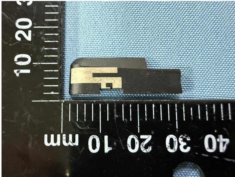
BLE/ANT+ Antenna
