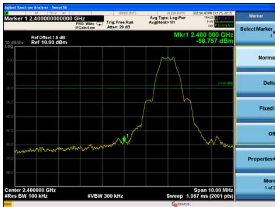
Channel 00 (2402MHz)-2
