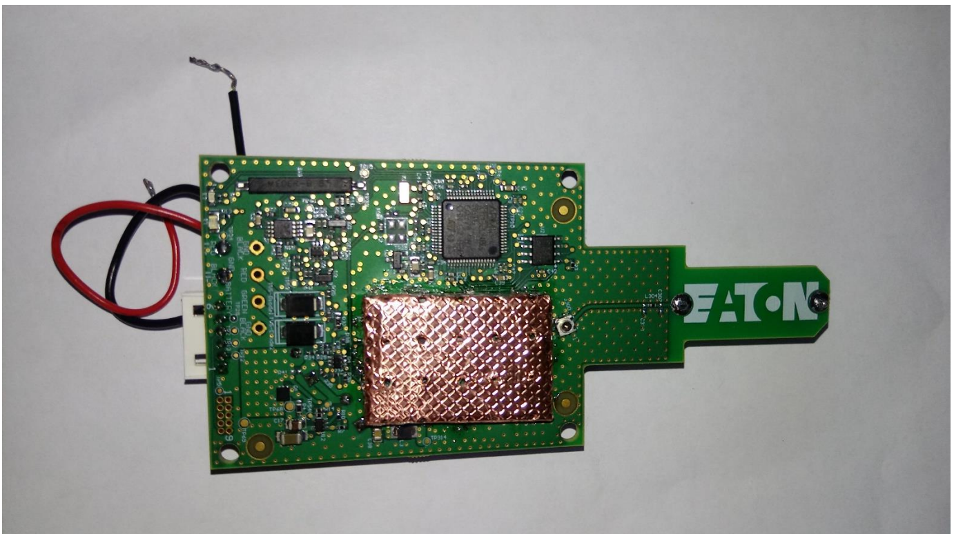
Figure 3: RFW-201 PCB – Top, Unpotted, Shield in Place
