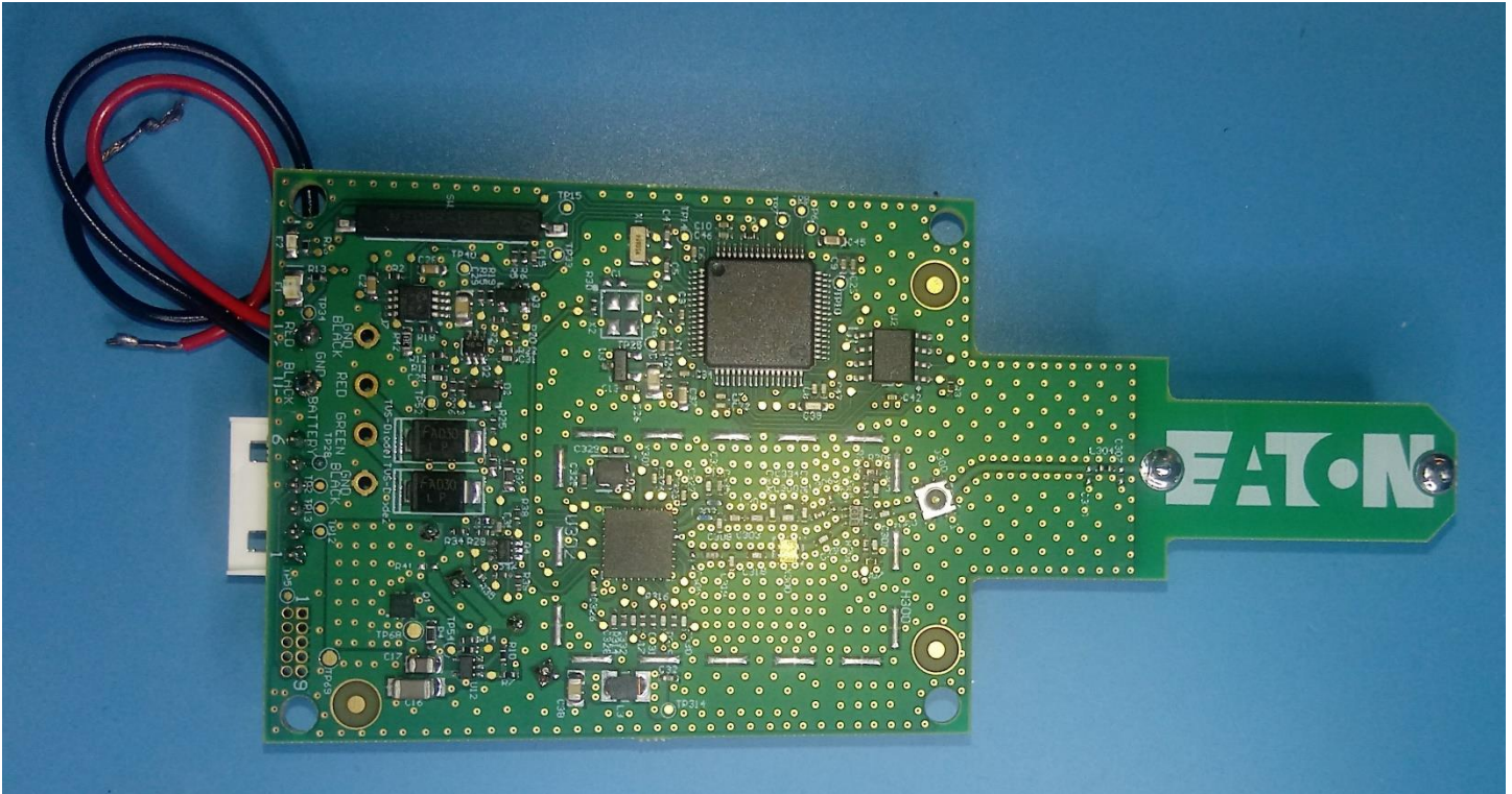
Figure 2: RFW-201 PCB – Top, Unpotted, Shield removed
