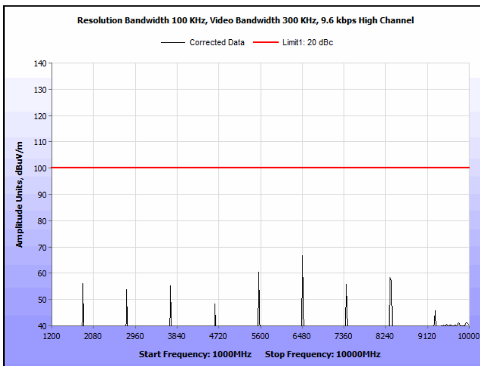
Plot 26. Radiated Spurious Emissions, High Channel, 9.6 kbps, 1 GHz – 10 GHz
