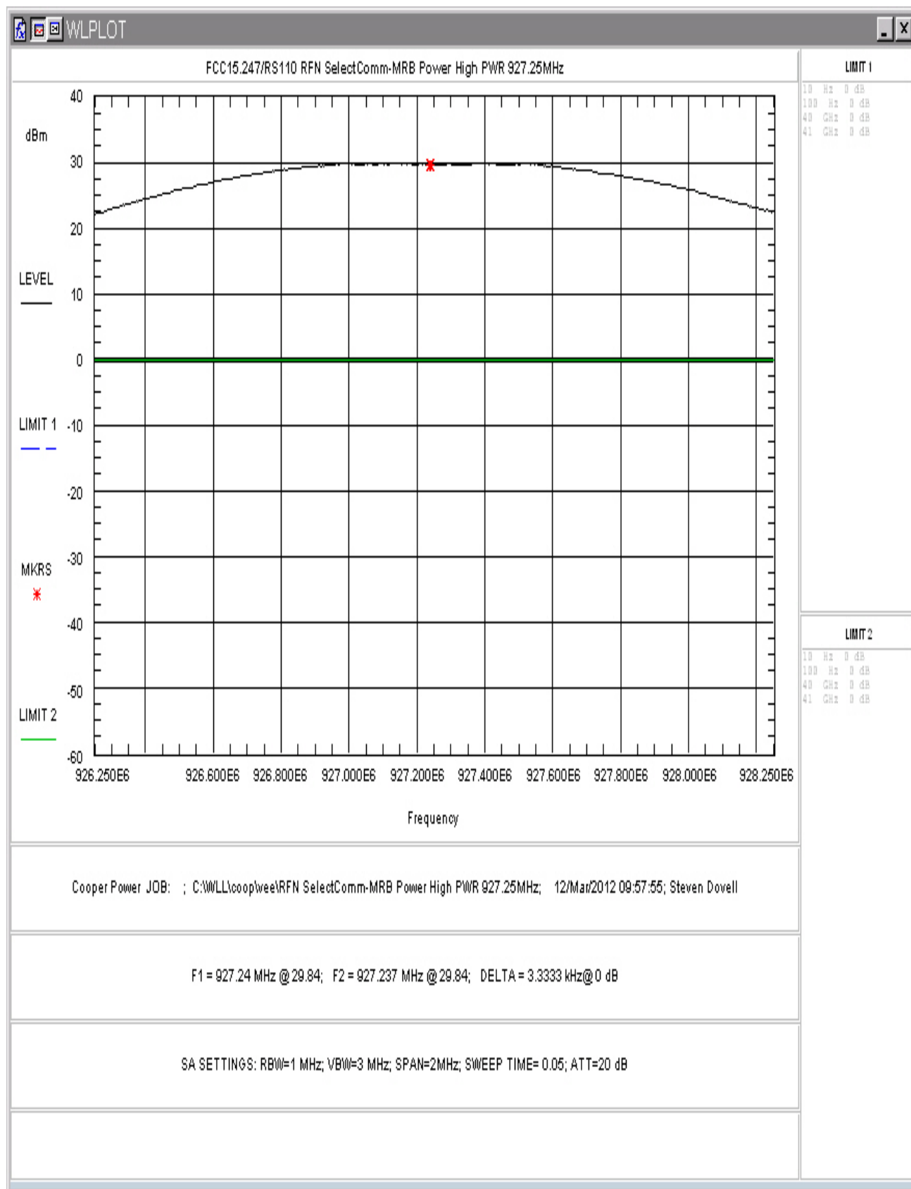
Figure 6: RF Peak Power, High Power, High Channel
