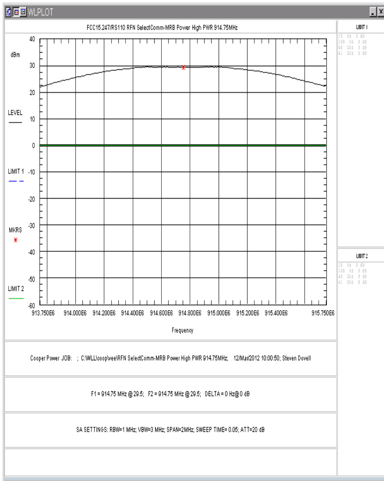
Figure 5: RF Peak Power, High Power, Center Channel
