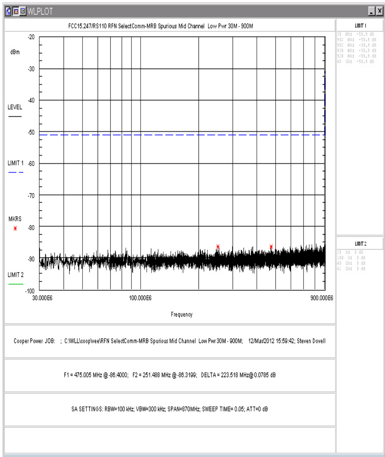
Figure 31: Conducted Spurious Emissions, Low Power, Center Channel 30 - 900MHz
