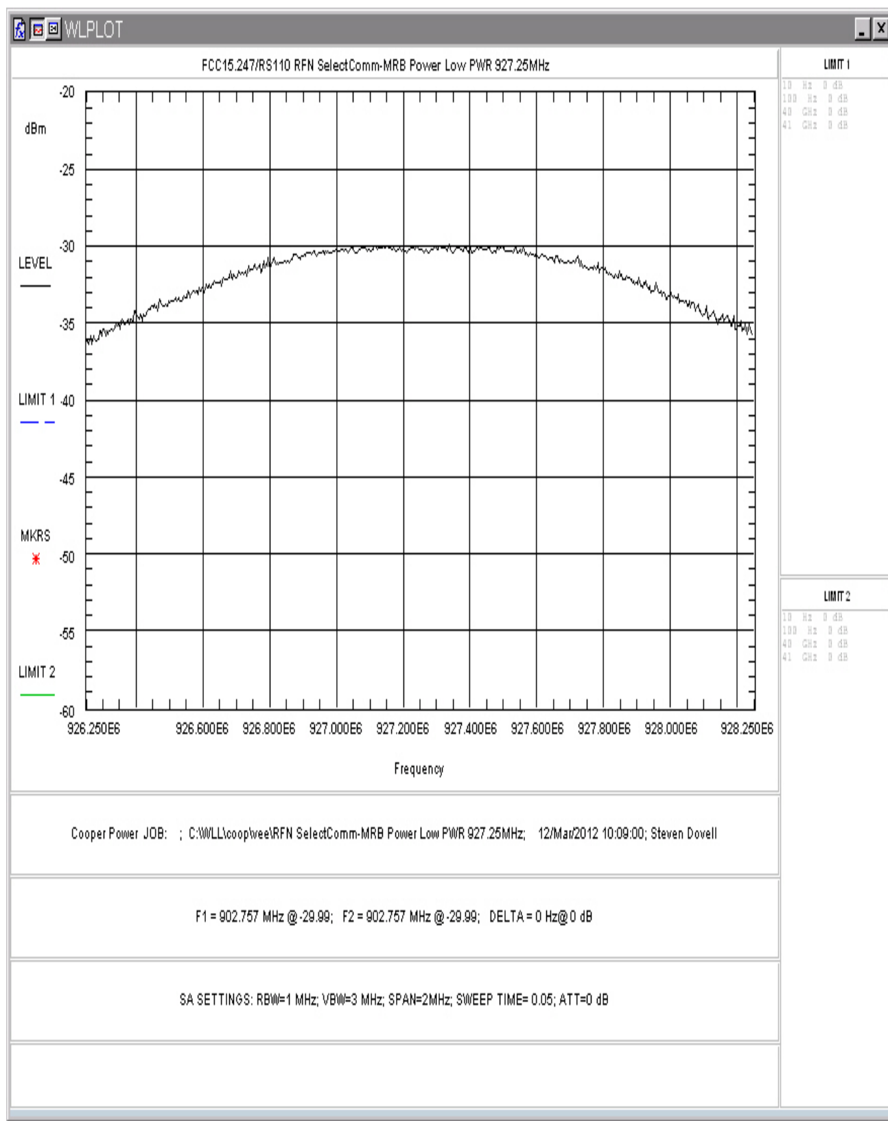
Figure 9: RF Peak Power, Low Power, High Channel
