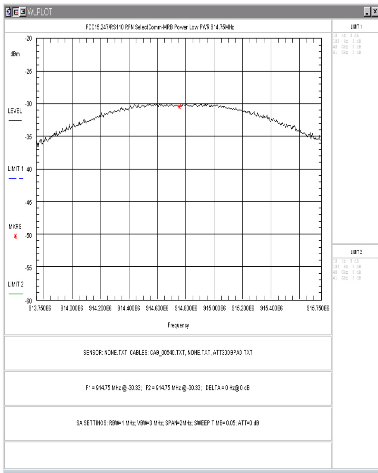
Figure 8: RF Peak Power, Low Power, Center Channel
