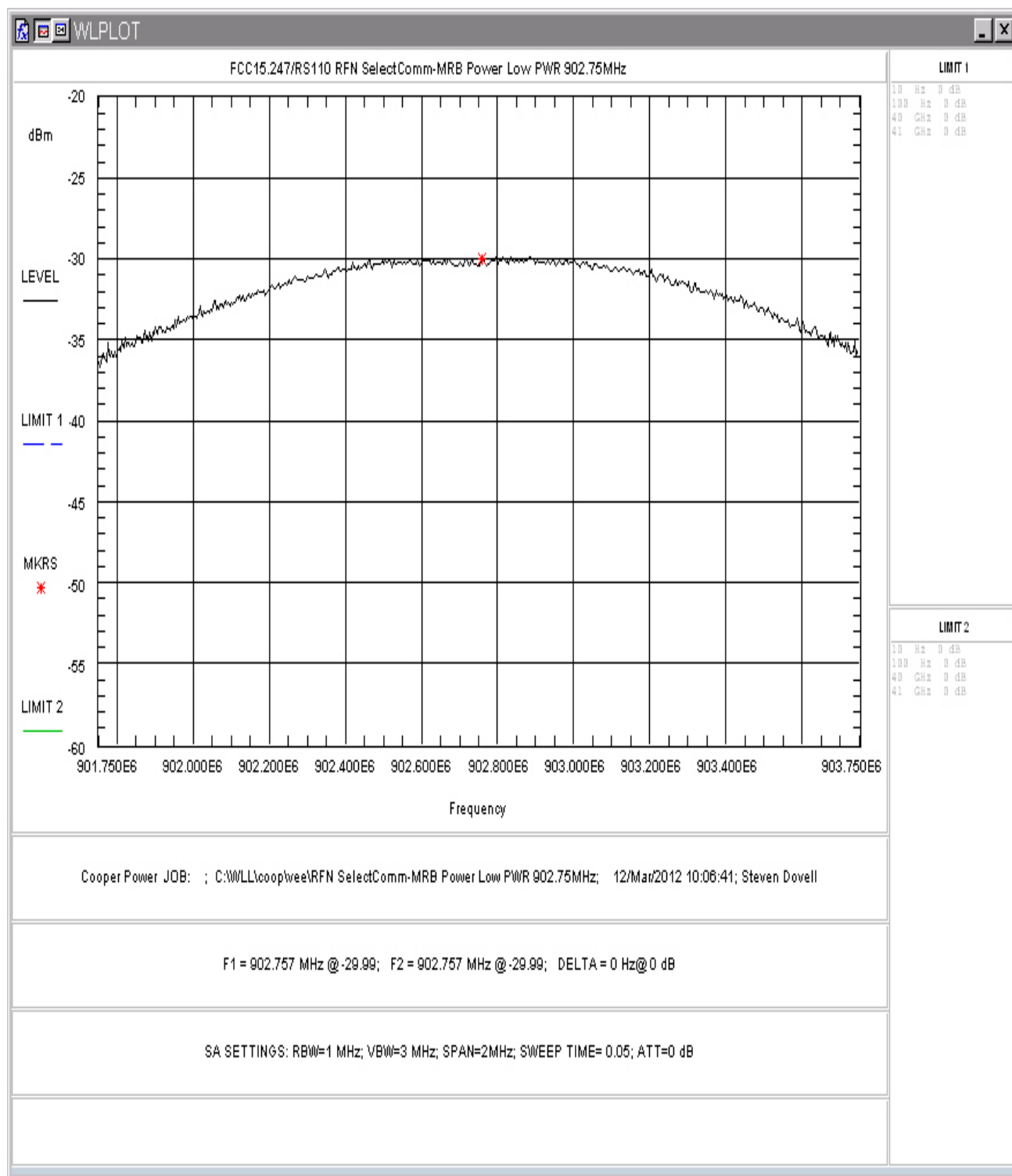
Figure 7: RF Peak Power, Low Power, Low Channel
