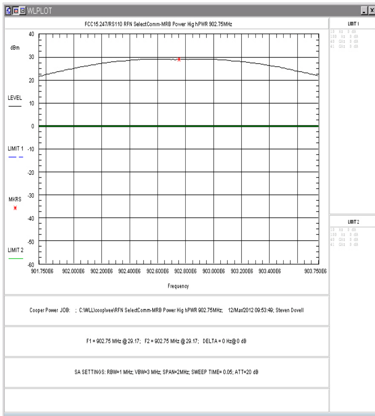
Figure 4: RF Peak Power, High Power, Low Channel
