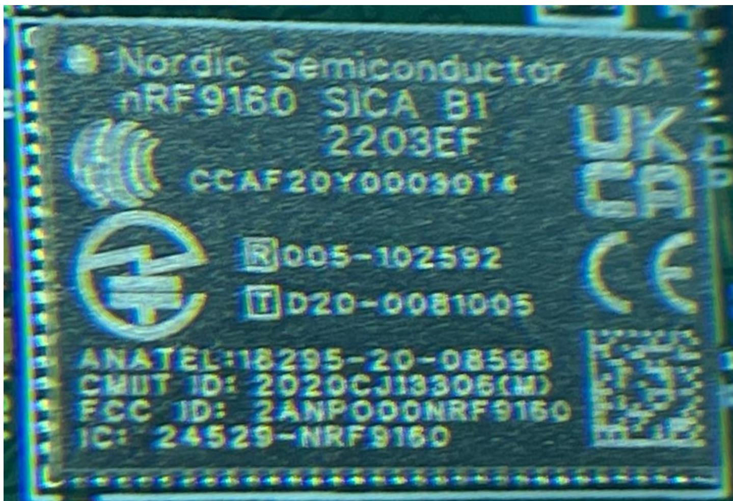
Cellular Chip (zoomed view) with FCC ID
