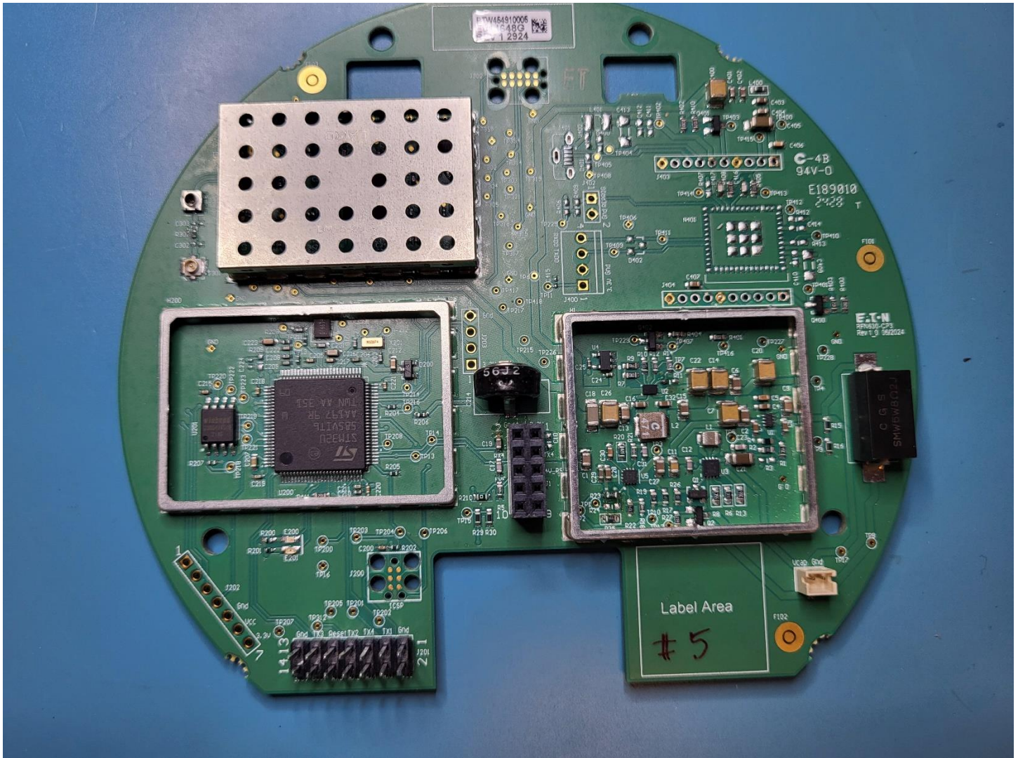
Figure 1: RFN-630CP3 PCB Top, RFN shield in place
