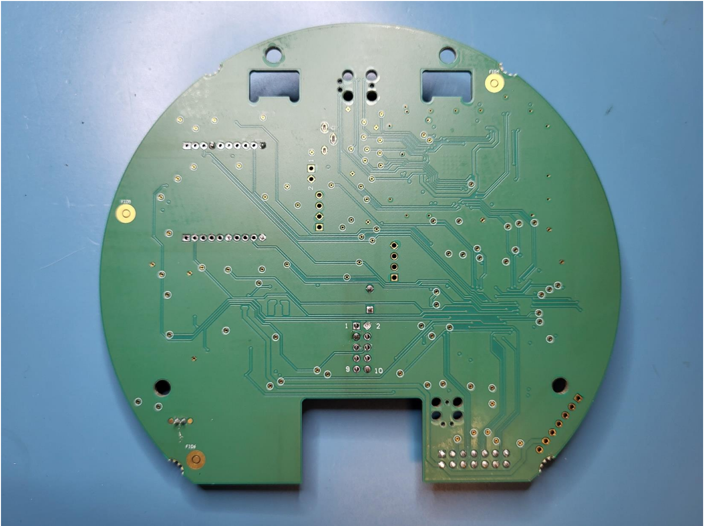
Figure 3: RFN-630CP3 PCB Bottom
