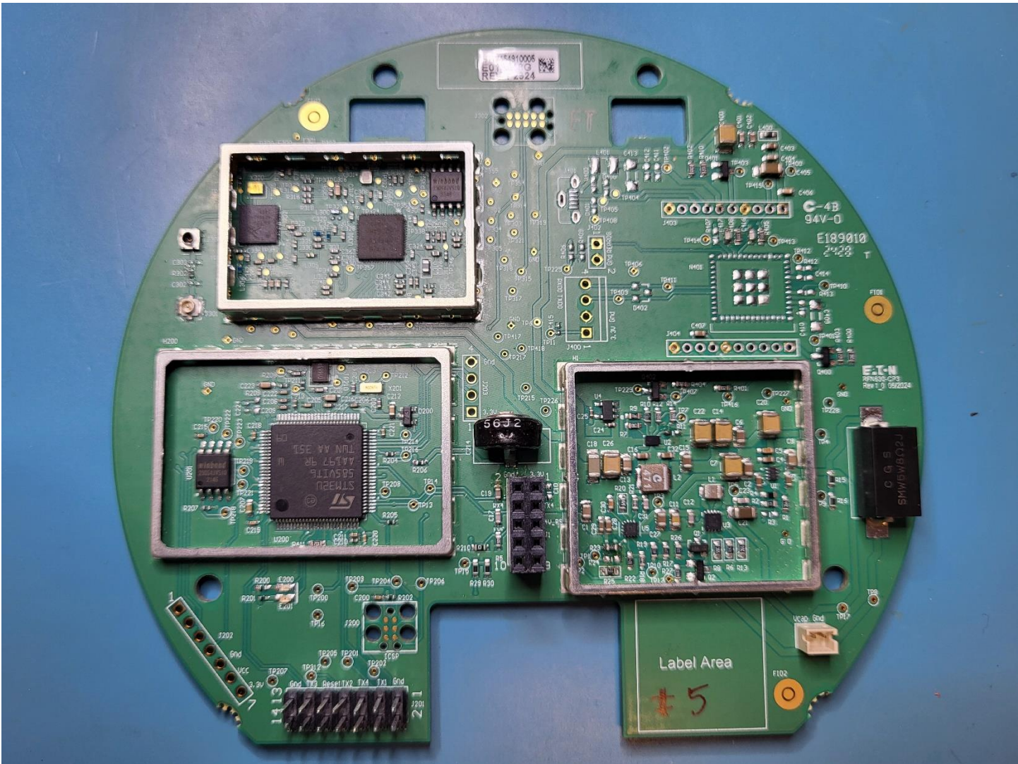
Figure 2: RFN-630CP3 PCB Top, RFN shield removed
