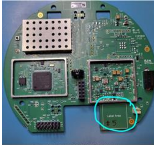
Figure 1: RFN-630CP3 PCB Top, RFN shield in place
